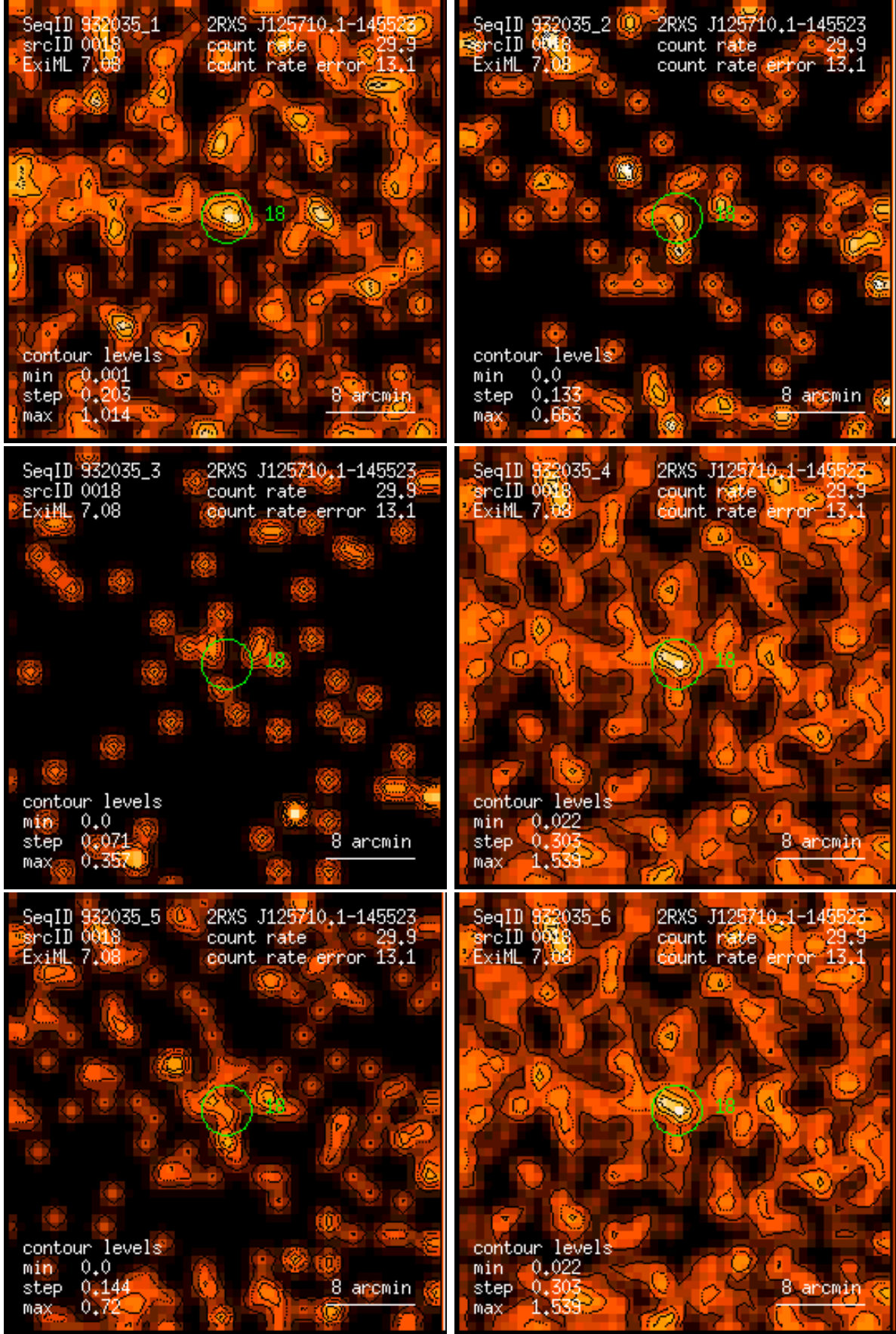
Figure 18: RASS 932035: detection 0018: band rate images, Gaussian filter: (1) PSPC channels 11 – 41, (2) 52 – 90, (3) 91 – 201, (4) 11 – 235, (5) 52 – 201, (6) 11 – 201. Broad band rates in counts/ks. Band rate contour levels in counts/ks/arcmin 2 .
