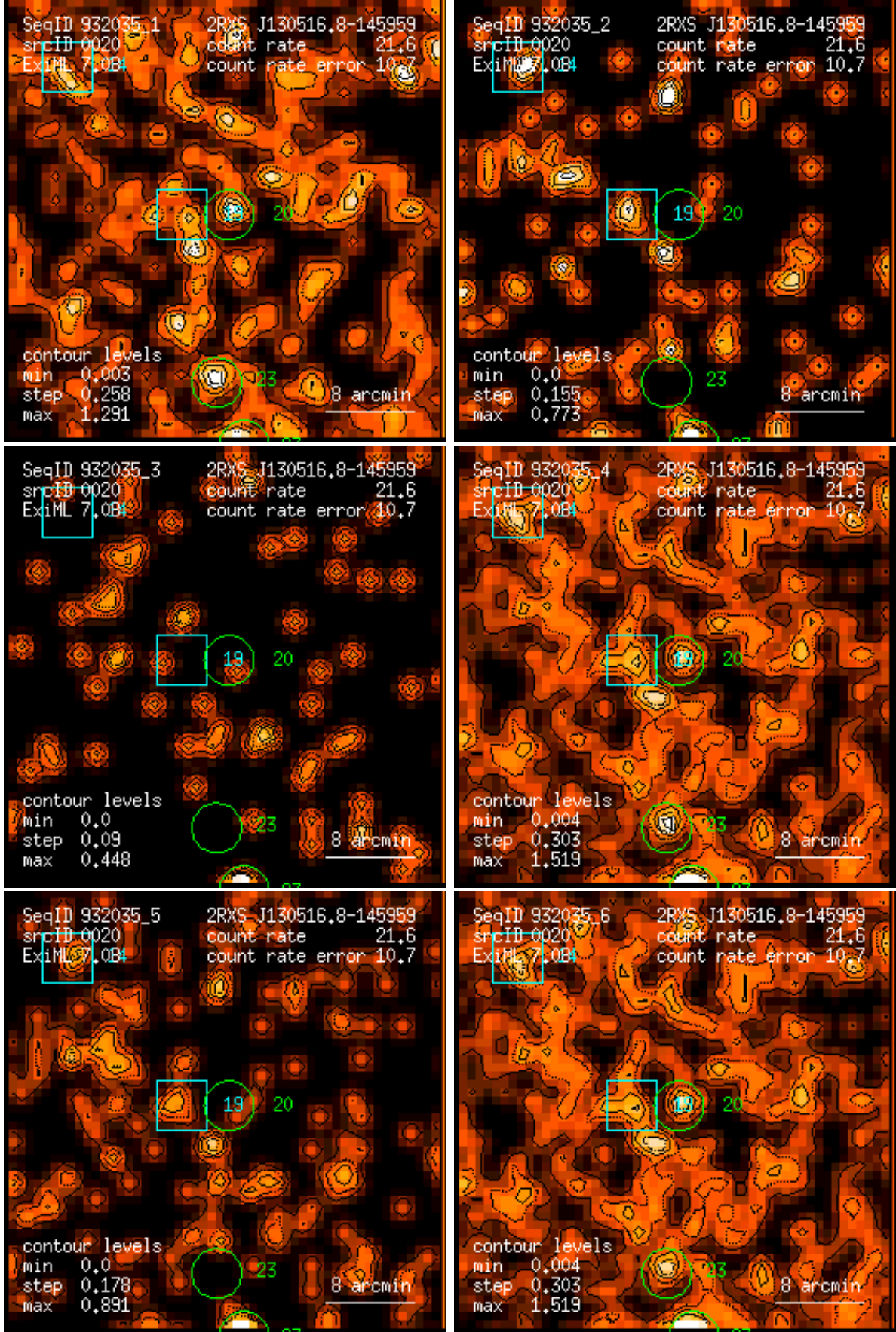
Figure 20: RASS 932035: detection 0020: band rate images, Gaussian filter: (1) PSPC channels 11 – 41, (2) 52 – 90, (3) 91 – 201, (4) 11 – 235, (5) 52 – 201, (6) 11 – 201. Broad band rates in counts/ks. Band rate contour levels in counts/ks/arcmin 2 .
