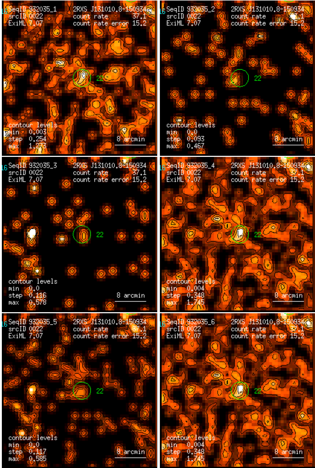
Figure 22: RASS 932035: detection 0022: band rate images, Gaussian filter: (1) PSPC channels 11 – 41, (2) 52 – 90, (3) 91 – 201, (4) 11 – 235, (5) 52 – 201, (6) 11 – 201. Broad band rates in counts/ks. Band rate contour levels in counts/ks/arcmin 2 .
