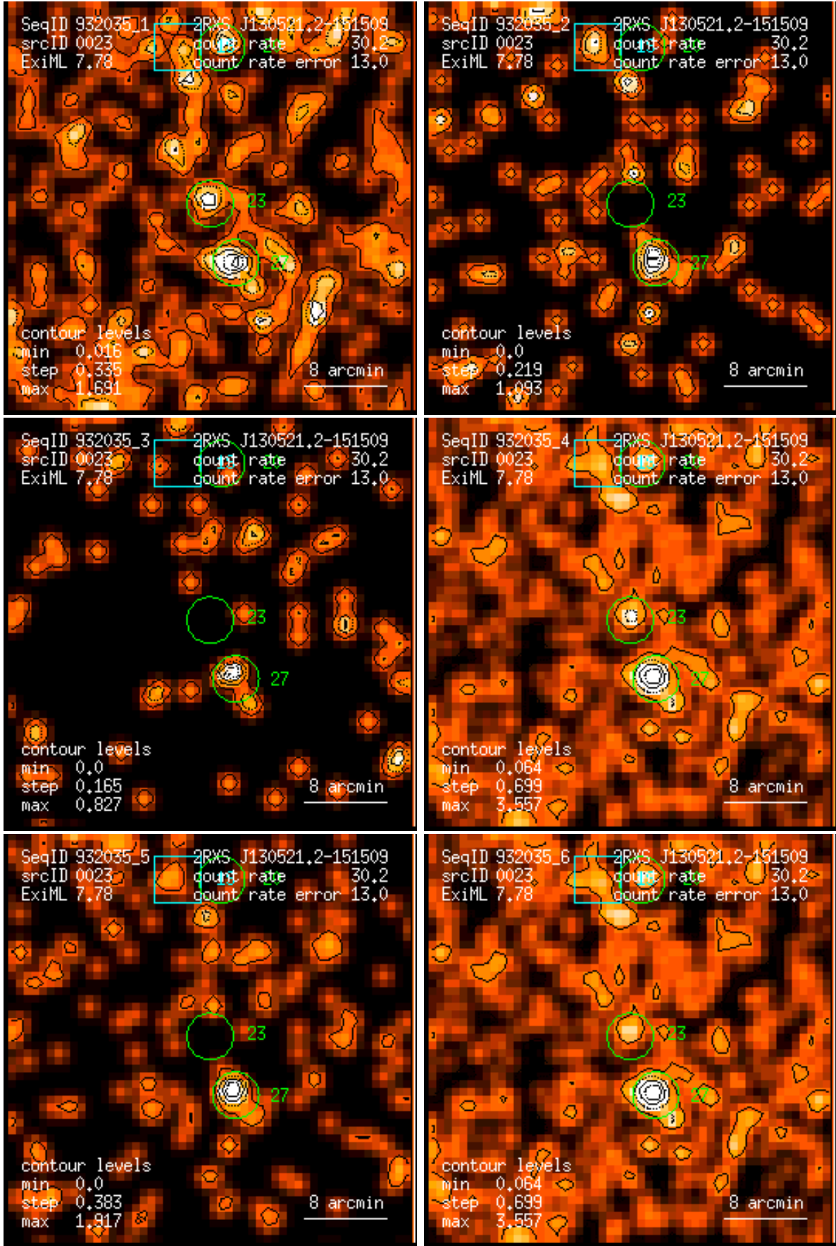
Figure 23: RASS 932035: detection 0023: band rate images, Gaussian filter: (1) PSPC channels 11 – 41, (2) 52 – 90, (3) 91 – 201, (4) 11 – 235, (5) 52 – 201, (6) 11 – 201. Broad band rates in counts/ks. Band rate contour levels in counts/ks/arcmin 2 .
