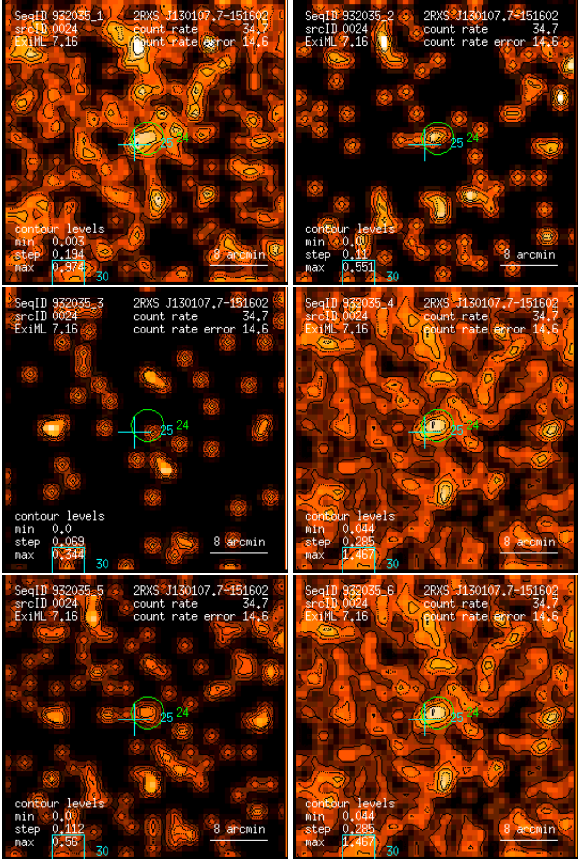
Figure 24: RASS 932035: detection 0024: band rate images, Gaussian filter: (1) PSPC channels 11 – 41, (2) 52 – 90, (3) 91 – 201, (4) 11 – 235, (5) 52 – 201, (6) 11 – 201. Broad band rates in counts/ks. Band rate contour levels in counts/ks/arcmin 2 .
