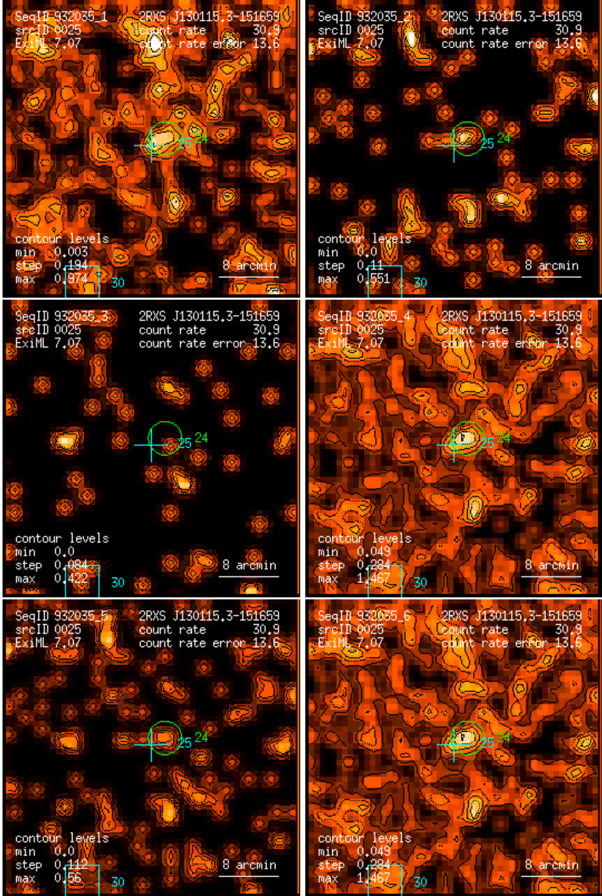
Figure 25: RASS 932035: detection 0025: band rate images, Gaussian filter: (1) PSPC channels 11 – 41, (2) 52 – 90, (3) 91 – 201, (4) 11 – 235, (5) 52 – 201, (6) 11 – 201. Broad band rates in counts/ks. Band rate contour levels in counts/ks/arcmin 2 .
