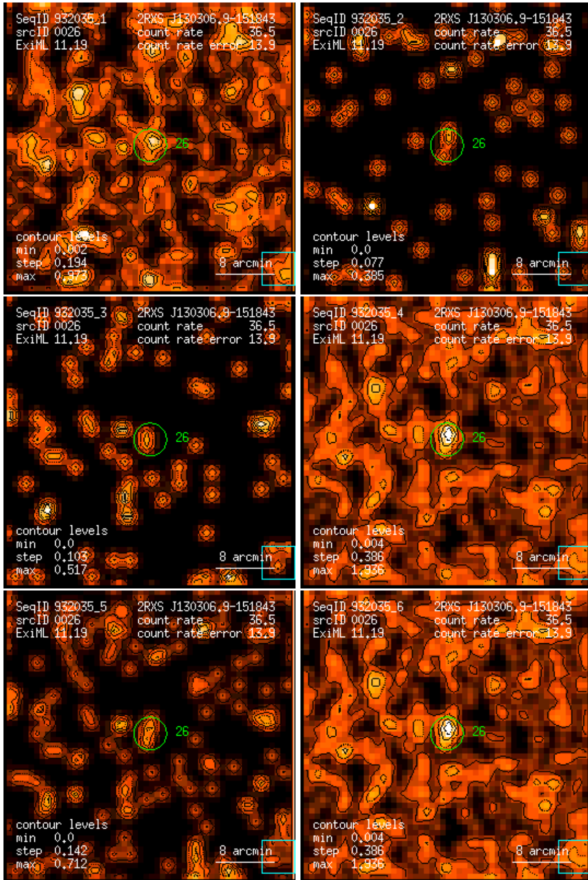
Figure 26: RASS 932035: detection 0026: band rate images, Gaussian filter: (1) PSPC channels 11 – 41, (2) 52 – 90, (3) 91 – 201, (4) 11 – 235, (5) 52 – 201, (6) 11 – 201. Broad band rates in counts/ks. Band rate contour levels in counts/ks/arcmin 2 .
