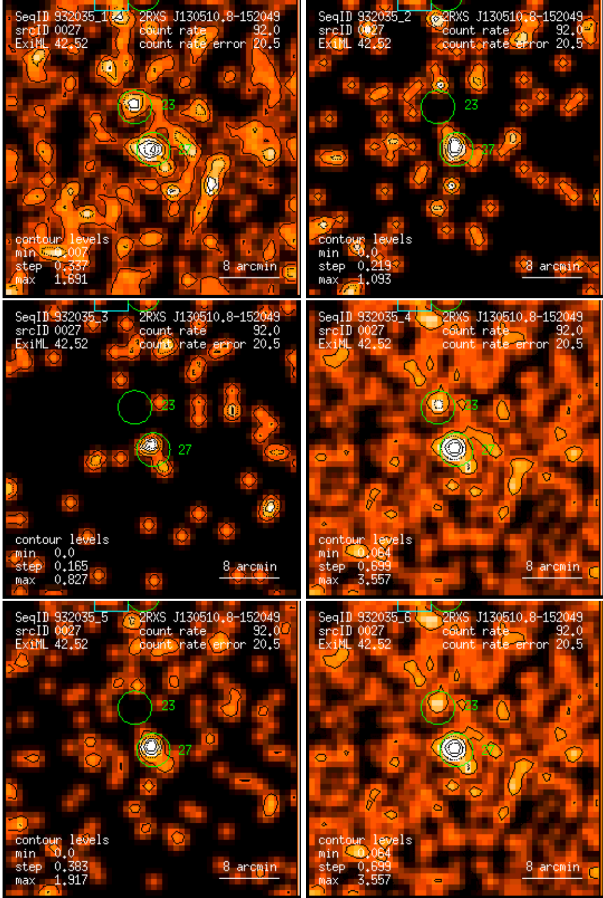
Figure 27: RASS 932035: detection 0027: band rate images, Gaussian filter: (1) PSPC channels 11 – 41, (2) 52 – 90, (3) 91 – 201, (4) 11 – 235, (5) 52 – 201, (6) 11 – 201. Broad band rates in counts/ks. Band rate contour levels in counts/ks/arcmin 2 .
