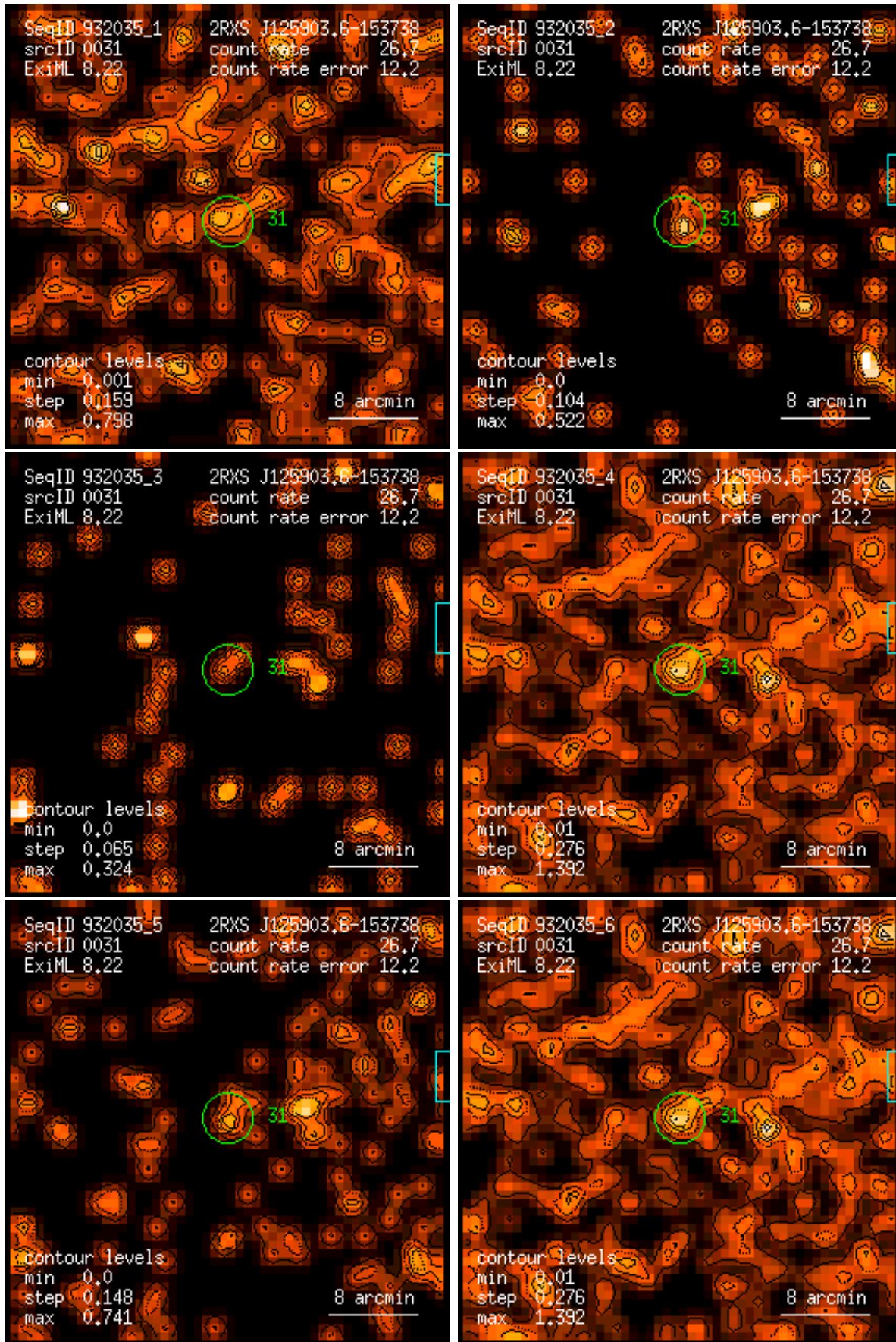
Figure 31: RASS 932035: detection 0031: band rate images, Gaussian filter: (1) PSPC channels 11 – 41, (2) 52 – 90, (3) 91 – 201, (4) 11 – 235, (5) 52 – 201, (6) 11 – 201. Broad band rates in counts/ks. Band rate contour levels in counts/ks/arcmin 2 .
