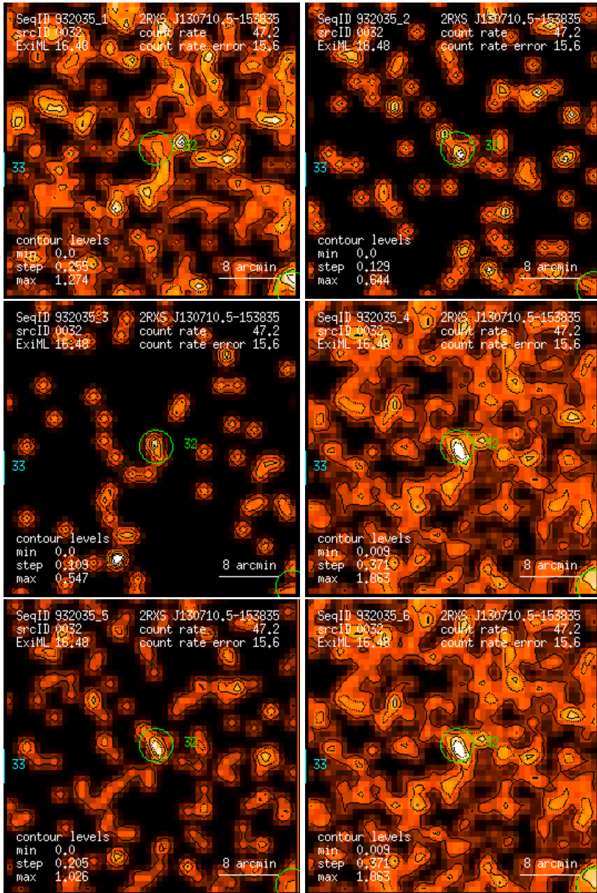
Figure 32: RASS 932035: detection 0032: band rate images, Gaussian filter: (1) PSPC channels 11 – 41, (2) 52 – 90, (3) 91 – 201, (4) 11 – 235, (5) 52 – 201, (6) 11 – 201. Broad band rates in counts/ks. Band rate contour levels in counts/ks/arcmin 2 .
