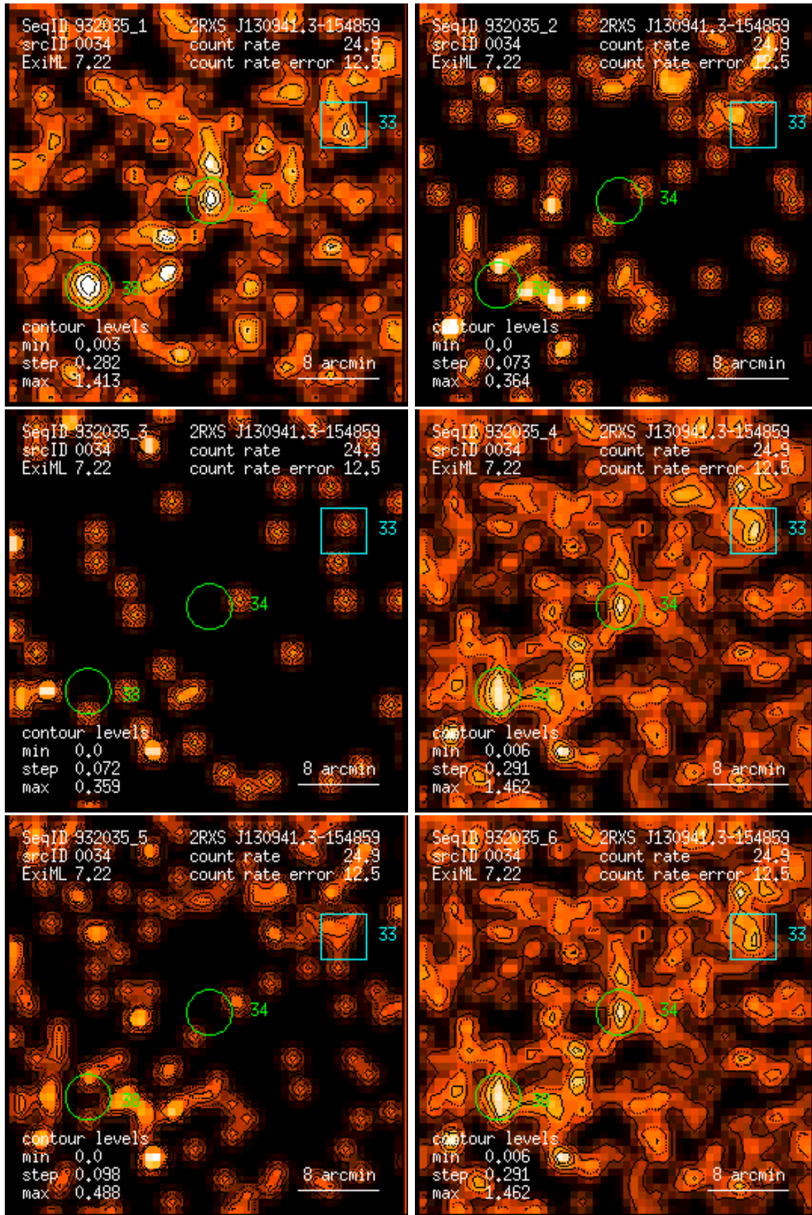
Figure 34: RASS 932035: detection 0034: band rate images, Gaussian filter: (1) PSPC channels 11 – 41, (2) 52 – 90, (3) 91 – 201, (4) 11 – 235, (5) 52 – 201, (6) 11 – 201. Broad band rates in counts/ks. Band rate contour levels in counts/ks/arcmin 2 .
