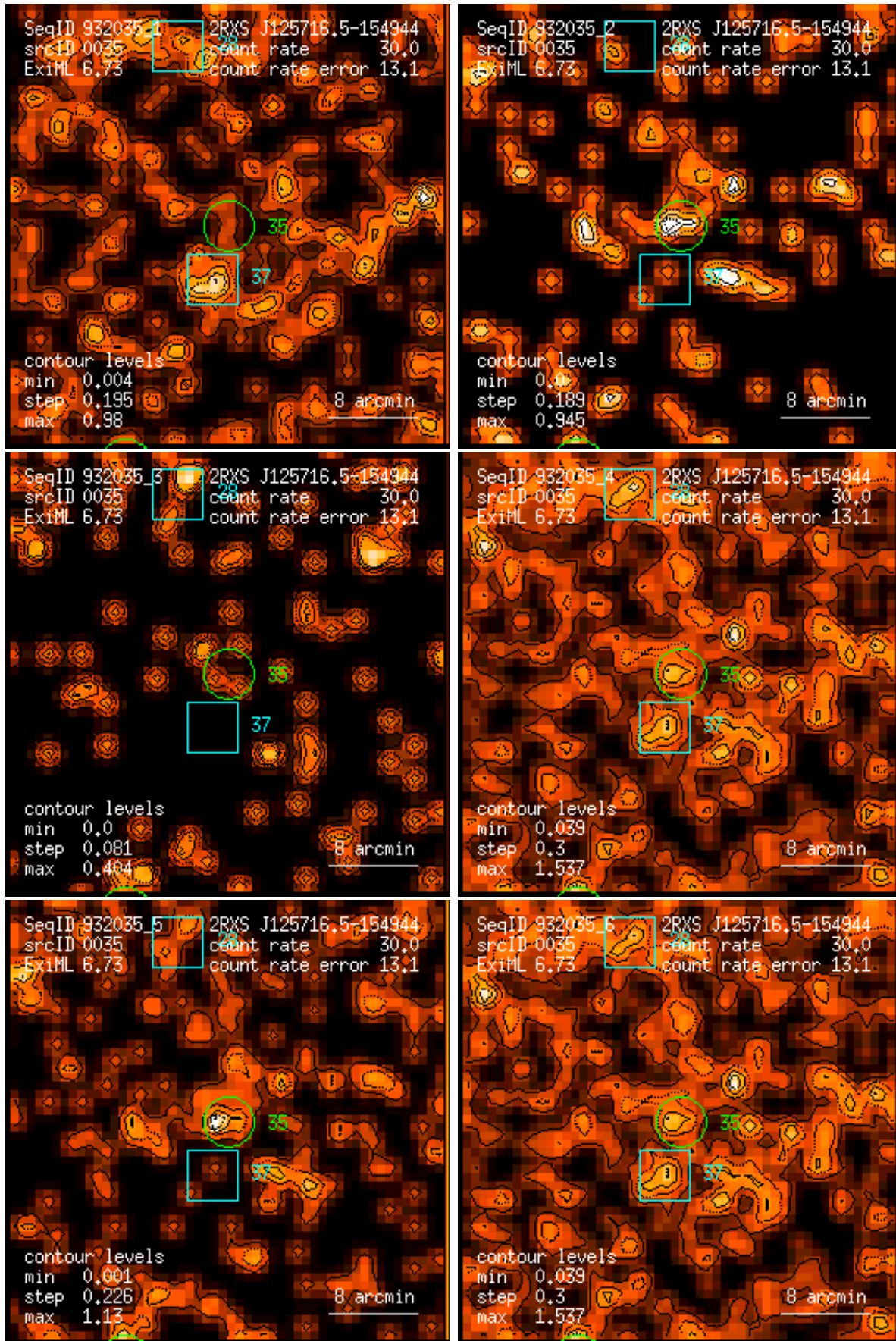
Figure 35: RASS 932035: detection 0035: band rate images, Gaussian filter: (1) PSPC channels 11 – 41, (2) 52 – 90, (3) 91 – 201, (4) 11 – 235, (5) 52 – 201, (6) 11 – 201. Broad band rates in counts/ks. Band rate contour levels in counts/ks/arcmin 2 .
