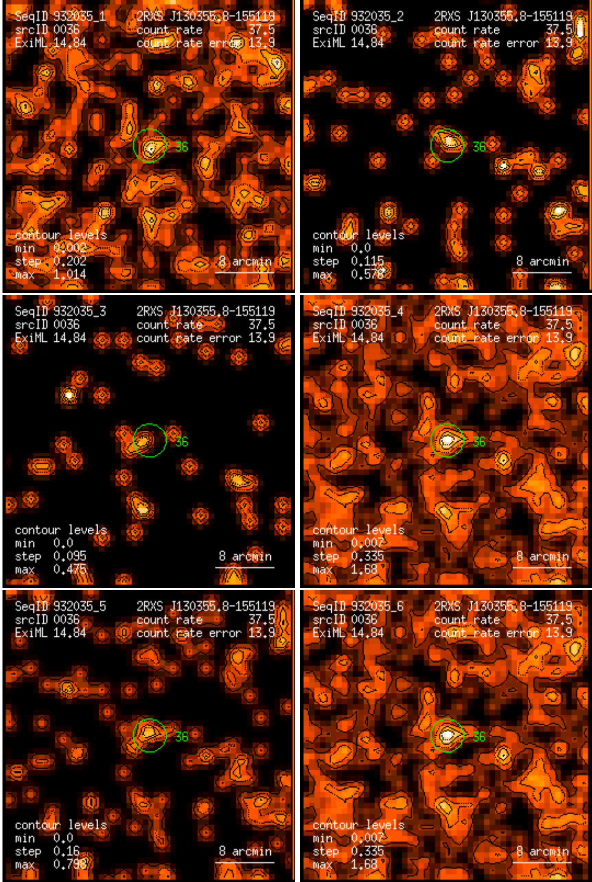
Figure 36: RASS 932035: detection 0036: band rate images, Gaussian filter: (1) PSPC channels 11 – 41, (2) 52 – 90, (3) 91 – 201, (4) 11 – 235, (5) 52 – 201, (6) 11 – 201. Broad band rates in counts/ks. Band rate contour levels in counts/ks/arcmin 2 .
