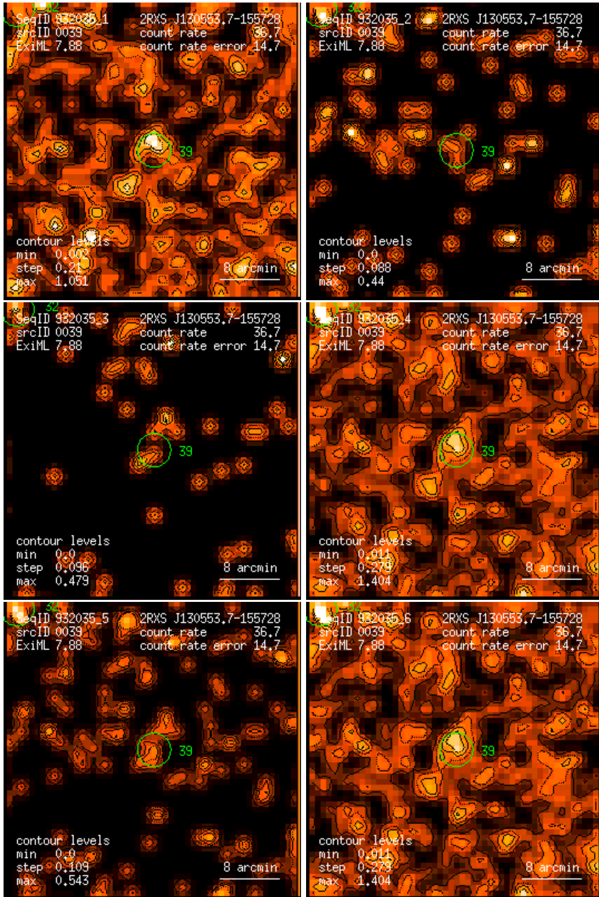
Figure 39: RASS 932035: detection 0039: band rate images, Gaussian filter: (1) PSPC channels 11 – 41, (2) 52 – 90, (3) 91 – 201, (4) 11 – 235, (5) 52 – 201, (6) 11 – 201. Broad band rates in counts/ks. Band rate contour levels in counts/ks/arcmin 2 .
