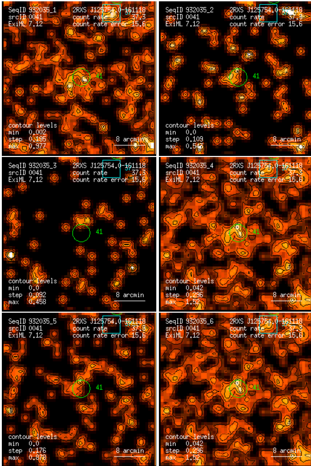
Figure 41: RASS 932035: detection 0041: band rate images, Gaussian filter: (1) PSPC channels 11 – 41, (2) 52 – 90, (3) 91 – 201, (4) 11 – 235, (5) 52 – 201, (6) 11 – 201. Broad band rates in counts/ks. Band rate contour levels in counts/ks/arcmin 2 .
