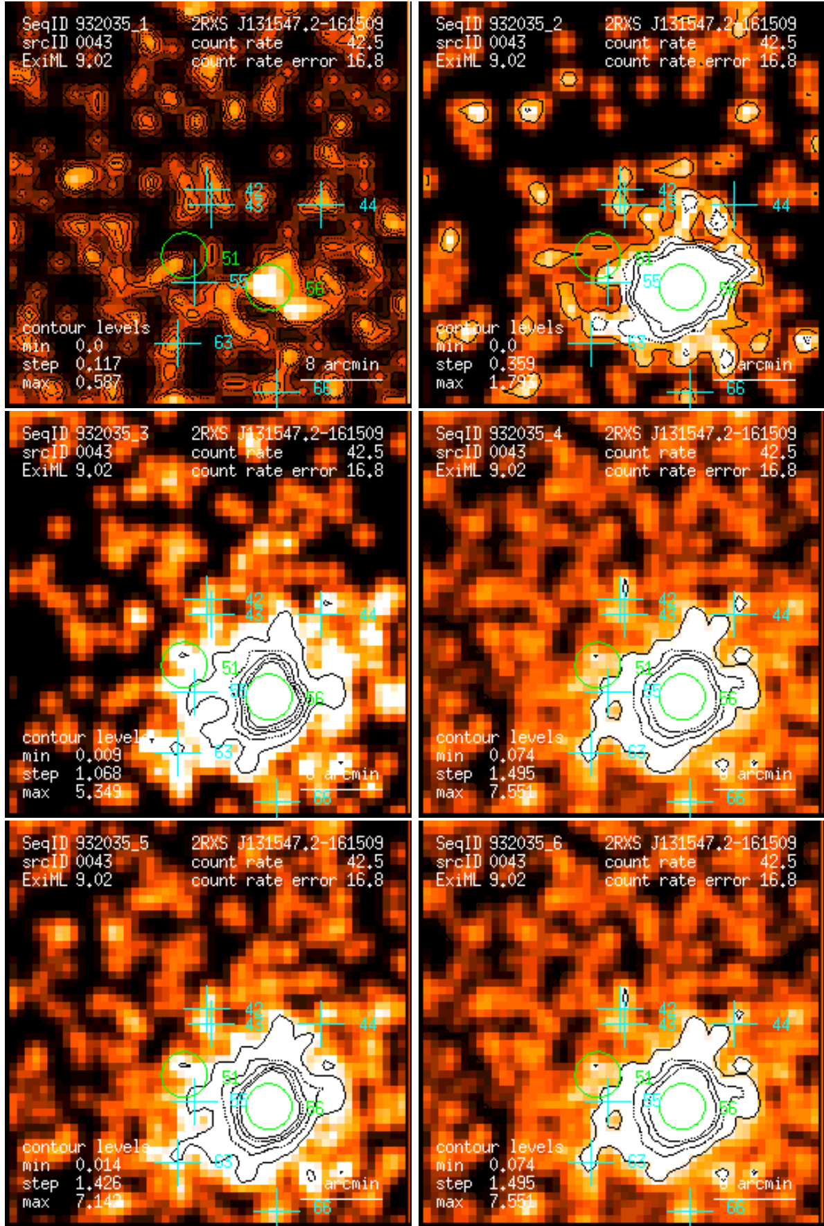
Figure 43: RASS 932035: detection 0043: band rate images, Gaussian filter: (1) PSPC channels 11 – 41, (2) 52 – 90, (3) 91 – 201, (4) 11 – 235, (5) 52 – 201, (6) 11 – 201. Broad band rates in counts/ks. Band rate contour levels in counts/ks/arcmin 2 .
