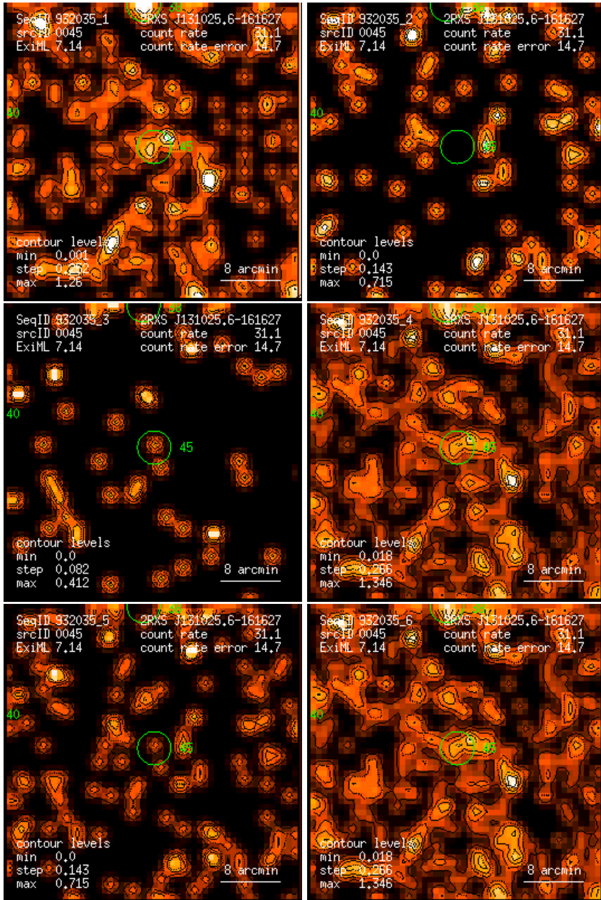
Figure 45: RASS 932035: detection 0045: band rate images, Gaussian filter: (1) PSPC channels 11 – 41, (2) 52 – 90, (3) 91 – 201, (4) 11 – 235, (5) 52 – 201, (6) 11 – 201. Broad band rates in counts/ks. Band rate contour levels in counts/ks/arcmin 2 .
