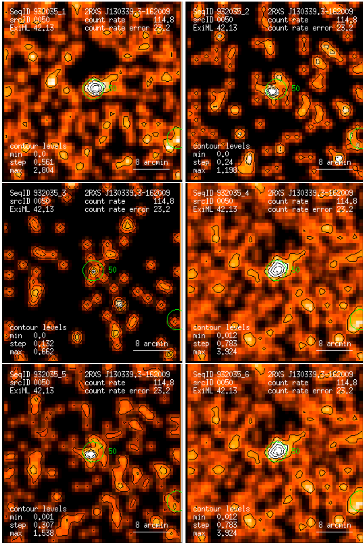
Figure 50: RASS 932035: detection 0050: band rate images, Gaussian filter: (1) PSPC channels 11 – 41, (2) 52 – 90, (3) 91 – 201, (4) 11 – 235, (5) 52 – 201, (6) 11 – 201. Broad band rates in counts/ks. Band rate contour levels in counts/ks/arcmin 2 .
