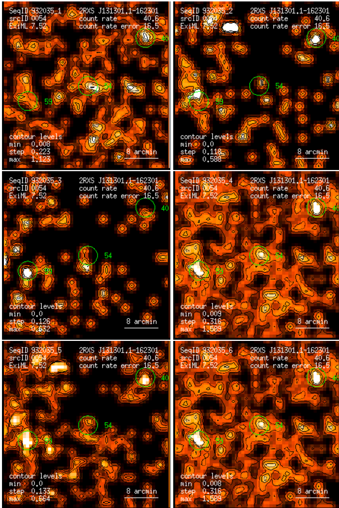
Figure 54: RASS 932035: detection 0054: band rate images, Gaussian filter: (1) PSPC channels 11 – 41, (2) 52 – 90, (3) 91 – 201, (4) 11 – 235, (5) 52 – 201, (6) 11 – 201. Broad band rates in counts/ks. Band rate contour levels in counts/ks/arcmin 2 .
