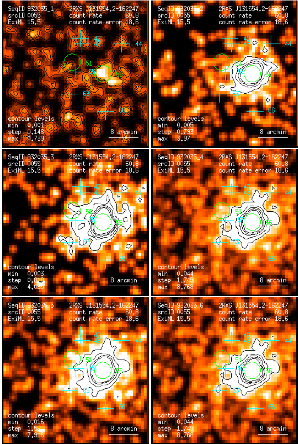
Figure 55: RASS 932035: detection 0055: band rate images, Gaussian filter: (1) PSPC channels 11 – 41, (2) 52 – 90, (3) 91 – 201, (4) 11 – 235, (5) 52 – 201, (6) 11 – 201. Broad band rates in counts/ks. Band rate contour levels in counts/ks/arcmin 2 .
