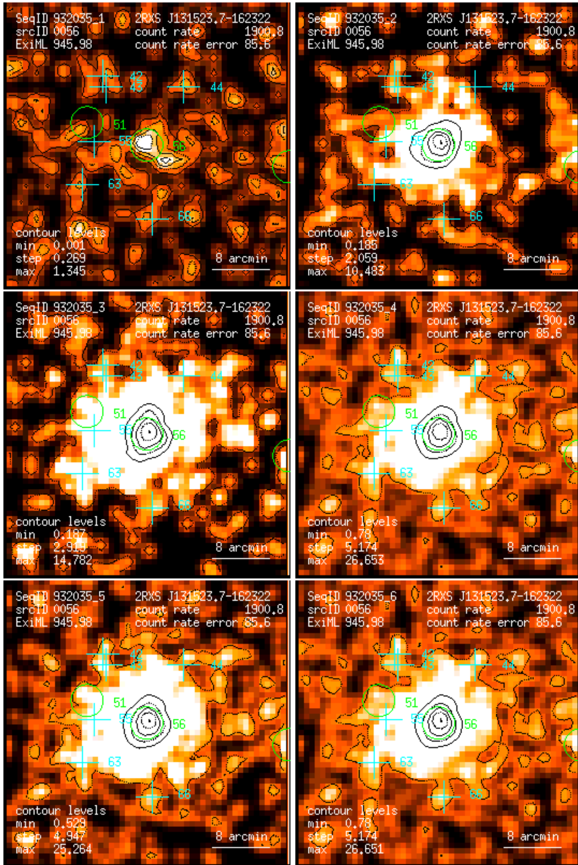
Figure 56: RASS 932035: detection 0056: band rate images, Gaussian filter: (1) PSPC channels 11 – 41, (2) 52 – 90, (3) 91 – 201, (4) 11 – 235, (5) 52 – 201, (6) 11 – 201. Broad band rates in counts/ks. Band rate contour levels in counts/ks/arcmin 2 .
