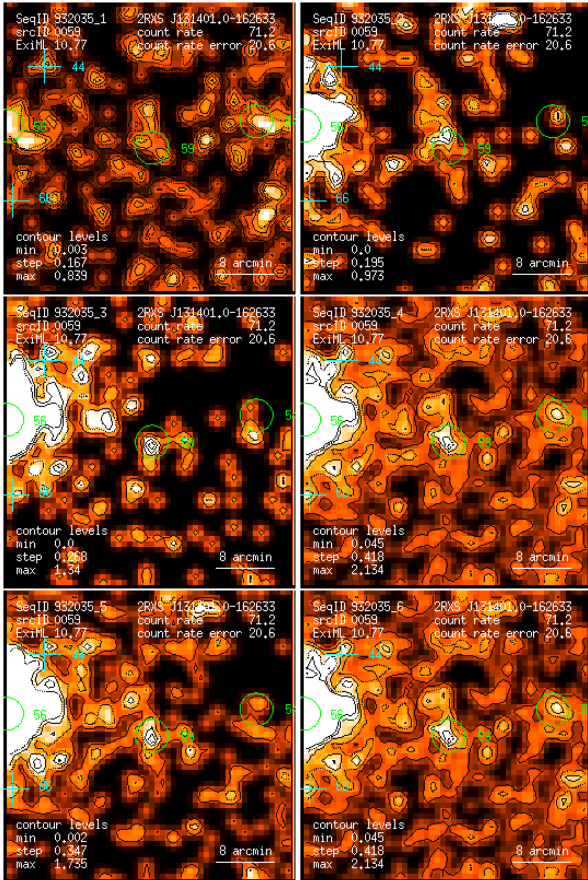
Figure 59: RASS 932035: detection 0059: band rate images, Gaussian filter: (1) PSPC channels 11 – 41, (2) 52 – 90, (3) 91 – 201, (4) 11 – 235, (5) 52 – 201, (6) 11 – 201. Broad band rates in counts/ks. Band rate contour levels in counts/ks/arcmin 2 .
