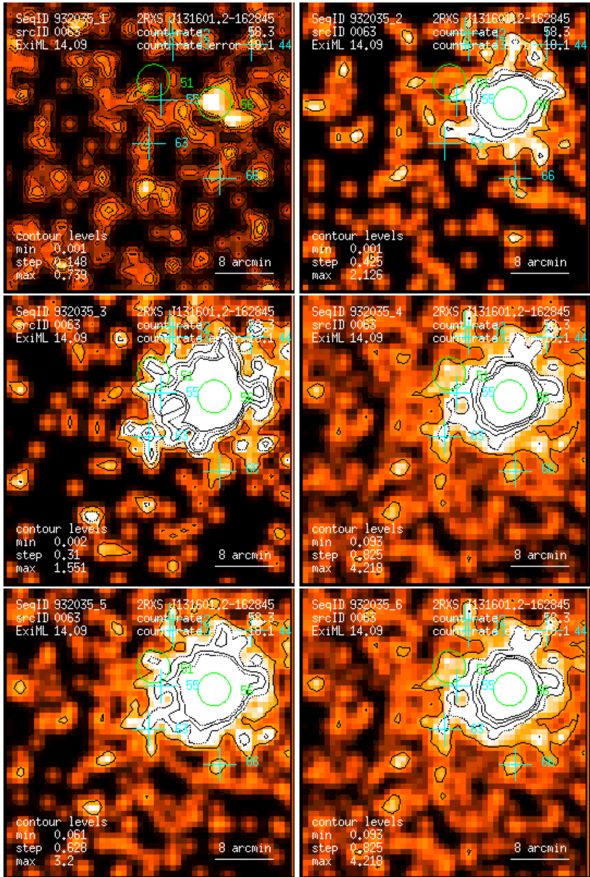
Figure 63: RASS 932035: detection 0063: band rate images, Gaussian filter: (1) PSPC channels 11 – 41, (2) 52 – 90, (3) 91 – 201, (4) 11 – 235, (5) 52 – 201, (6) 11 – 201. Broad band rates in counts/ks. Band rate contour levels in counts/ks/arcmin 2 .
