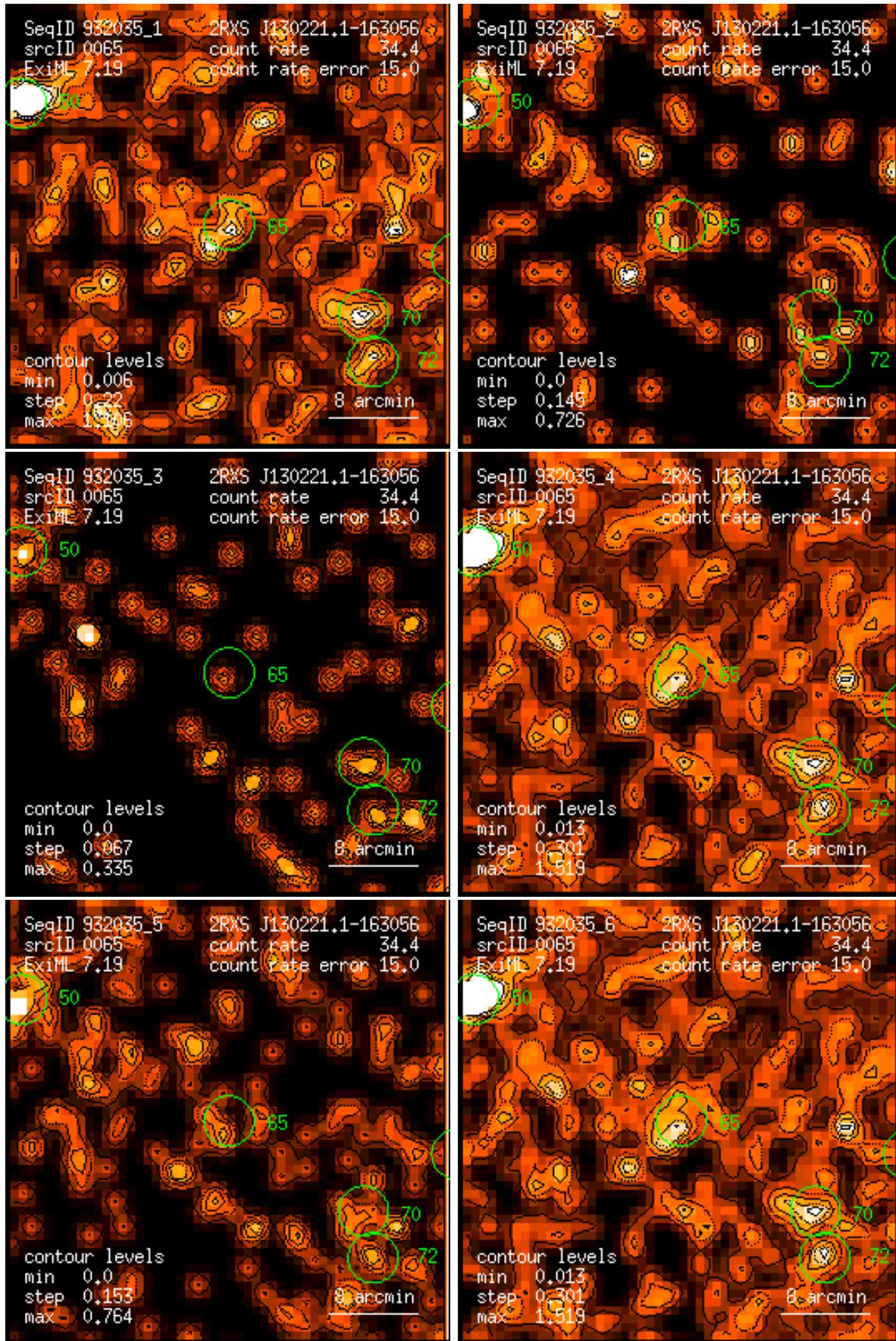
Figure 65: RASS 932035: detection 0065: band rate images, Gaussian filter: (1) PSPC channels 11 – 41, (2) 52 – 90, (3) 91 – 201, (4) 11 – 235, (5) 52 – 201, (6) 11 – 201. Broad band rates in counts/ks. Band rate contour levels in counts/ks/arcmin 2 .
