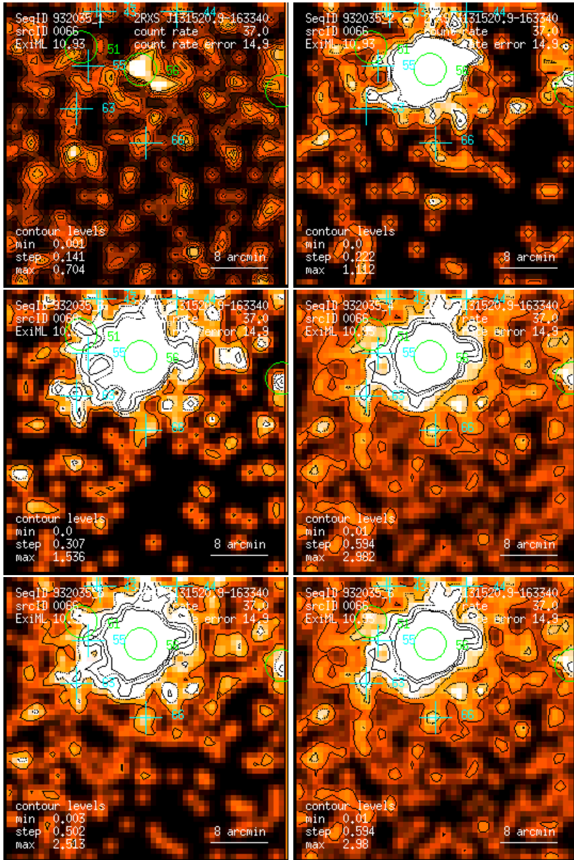
Figure 66: RASS 932035: detection 0066: band rate images, Gaussian filter: (1) PSPC channels 11 – 41, (2) 52 – 90, (3) 91 – 201, (4) 11 – 235, (5) 52 – 201, (6) 11 – 201. Broad band rates in counts/ks. Band rate contour levels in counts/ks/arcmin 2 .
