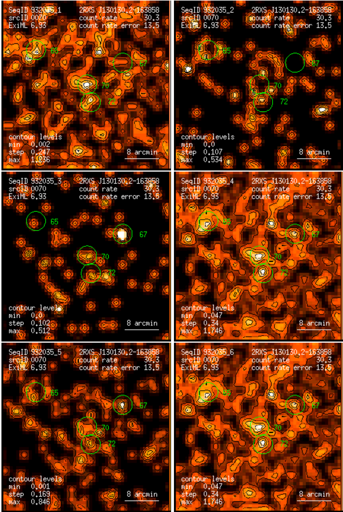
Figure 70: RASS 932035: detection 0070: band rate images, Gaussian filter: (1) PSPC channels 11 – 41, (2) 52 – 90, (3) 91 – 201, (4) 11 – 235, (5) 52 – 201, (6) 11 – 201. Broad band rates in counts/ks. Band rate contour levels in counts/ks/arcmin 2 .
