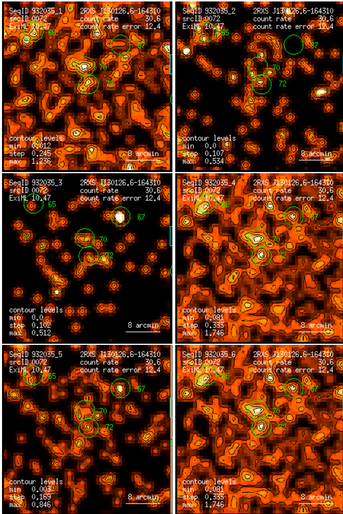
Figure 72: RASS 932035: detection 0072: band rate images, Gaussian filter: (1) PSPC channels 11 – 41, (2) 52 – 90, (3) 91 – 201, (4) 11 – 235, (5) 52 – 201, (6) 11 – 201. Broad band rates in counts/ks. Band rate contour levels in counts/ks/arcmin 2 .
