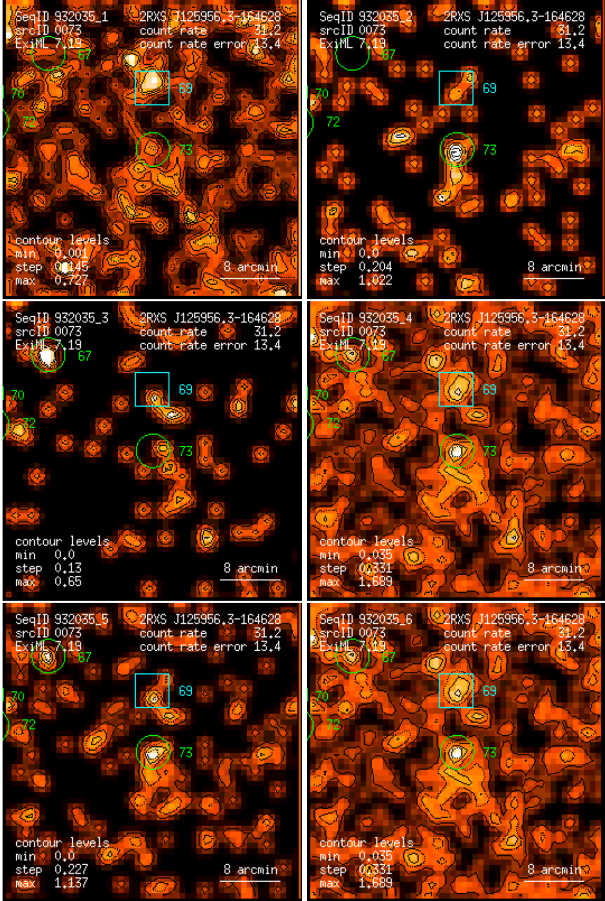
Figure 73: RASS 932035: detection 0073: band rate images, Gaussian filter: (1) PSPC channels 11 – 41, (2) 52 – 90, (3) 91 – 201, (4) 11 – 235, (5) 52 – 201, (6) 11 – 201. Broad band rates in counts/ks. Band rate contour levels in counts/ks/arcmin 2 .
