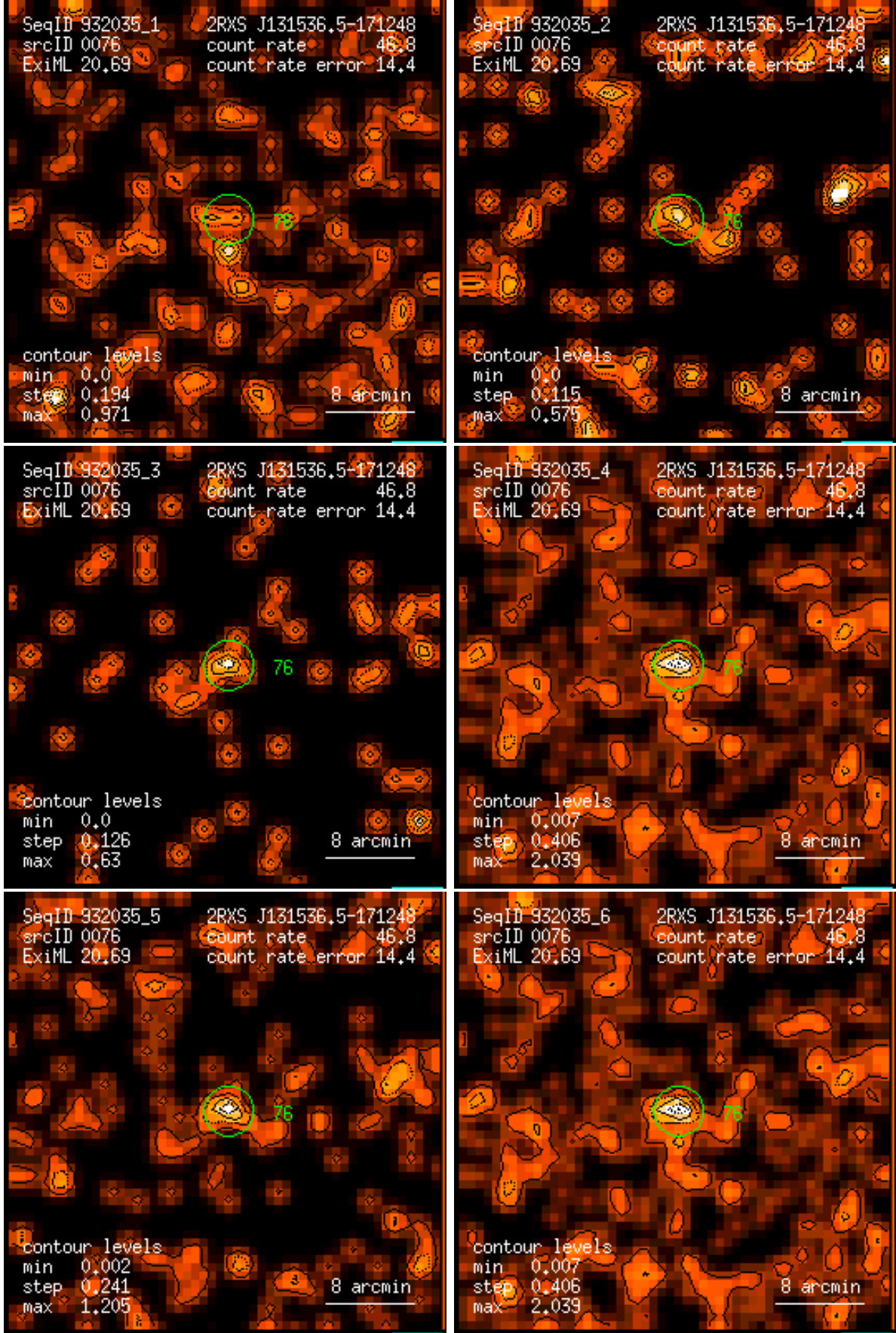
Figure 76: RASS 932035: detection 0076: band rate images, Gaussian filter: (1) PSPC channels 11 – 41, (2) 52 – 90, (3) 91 – 201, (4) 11 – 235, (5) 52 – 201, (6) 11 – 201. Broad band rates in counts/ks. Band rate contour levels in counts/ks/arcmin 2 .
