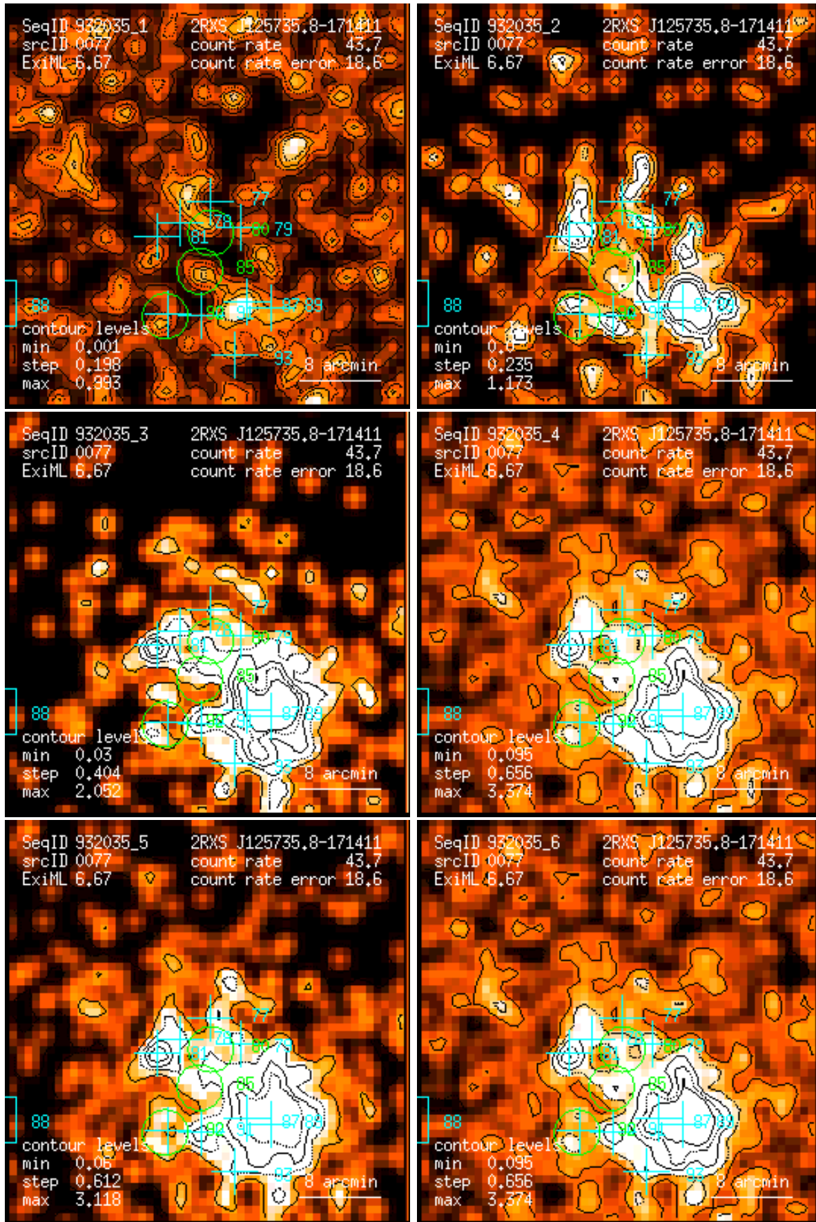
Figure 77: RASS 932035: detection 0077: band rate images, Gaussian filter: (1) PSPC channels 11 – 41, (2) 52 – 90, (3) 91 – 201, (4) 11 – 235, (5) 52 – 201, (6) 11 – 201. Broad band rates in counts/ks. Band rate contour levels in counts/ks/arcmin 2 .
