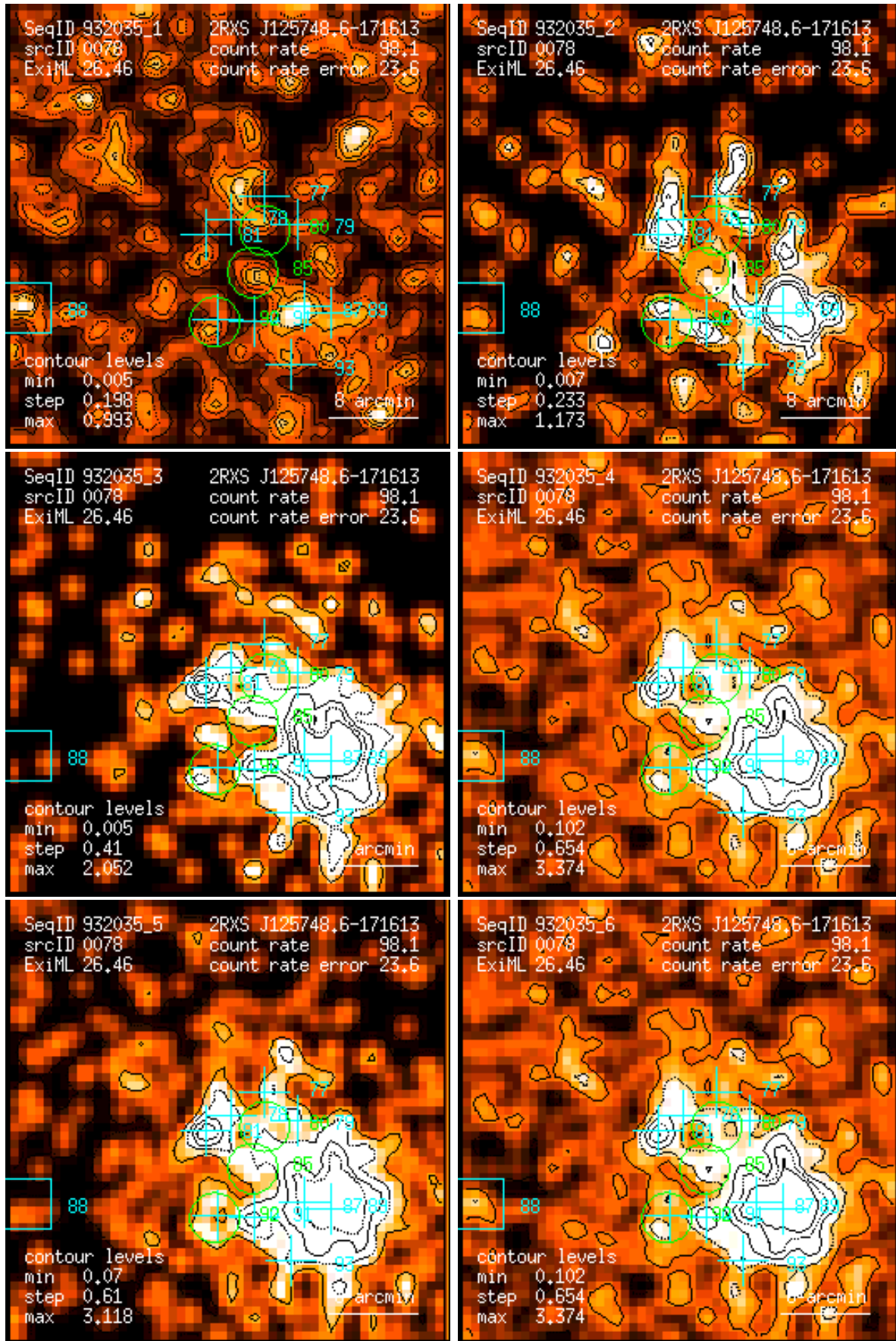
Figure 78: RASS 932035: detection 0078: band rate images, Gaussian filter: (1) PSPC channels 11 – 41, (2) 52 – 90, (3) 91 – 201, (4) 11 – 235, (5) 52 – 201, (6) 11 – 201. Broad band rates in counts/ks. Band rate contour levels in counts/ks/arcmin 2 .
