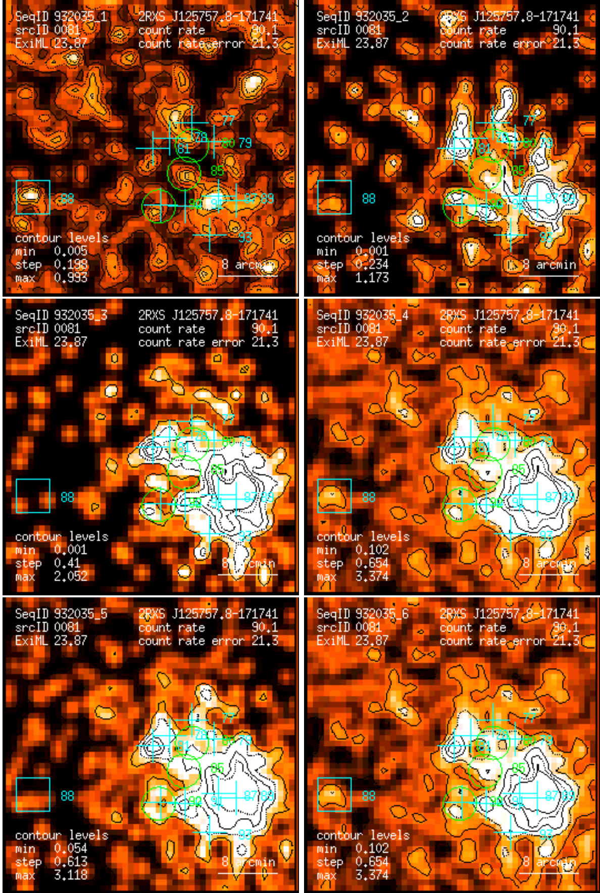
Figure 81: RASS 932035: detection 0081: band rate images, Gaussian filter: (1) PSPC channels 11 – 41, (2) 52 – 90, (3) 91 – 201, (4) 11 – 235, (5) 52 – 201, (6) 11 – 201. Broad band rates in counts/ks. Band rate contour levels in counts/ks/arcmin 2 .
