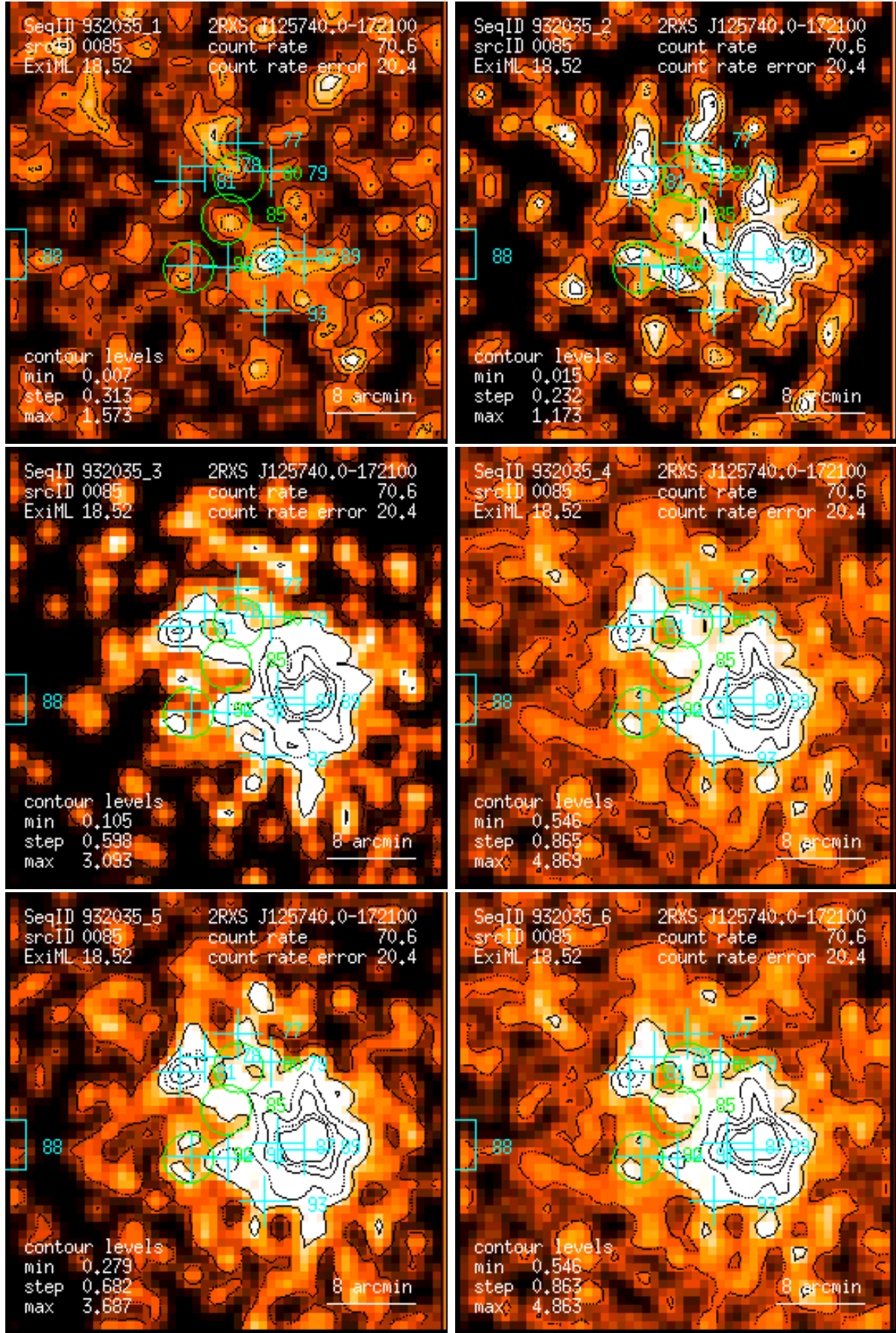
Figure 85: RASS 932035: detection 0085: band rate images, Gaussian filter: (1) PSPC channels 11 – 41, (2) 52 – 90, (3) 91 – 201, (4) 11 – 235, (5) 52 – 201, (6) 11 – 201. Broad band rates in counts/ks. Band rate contour levels in counts/ks/arcmin 2 .
