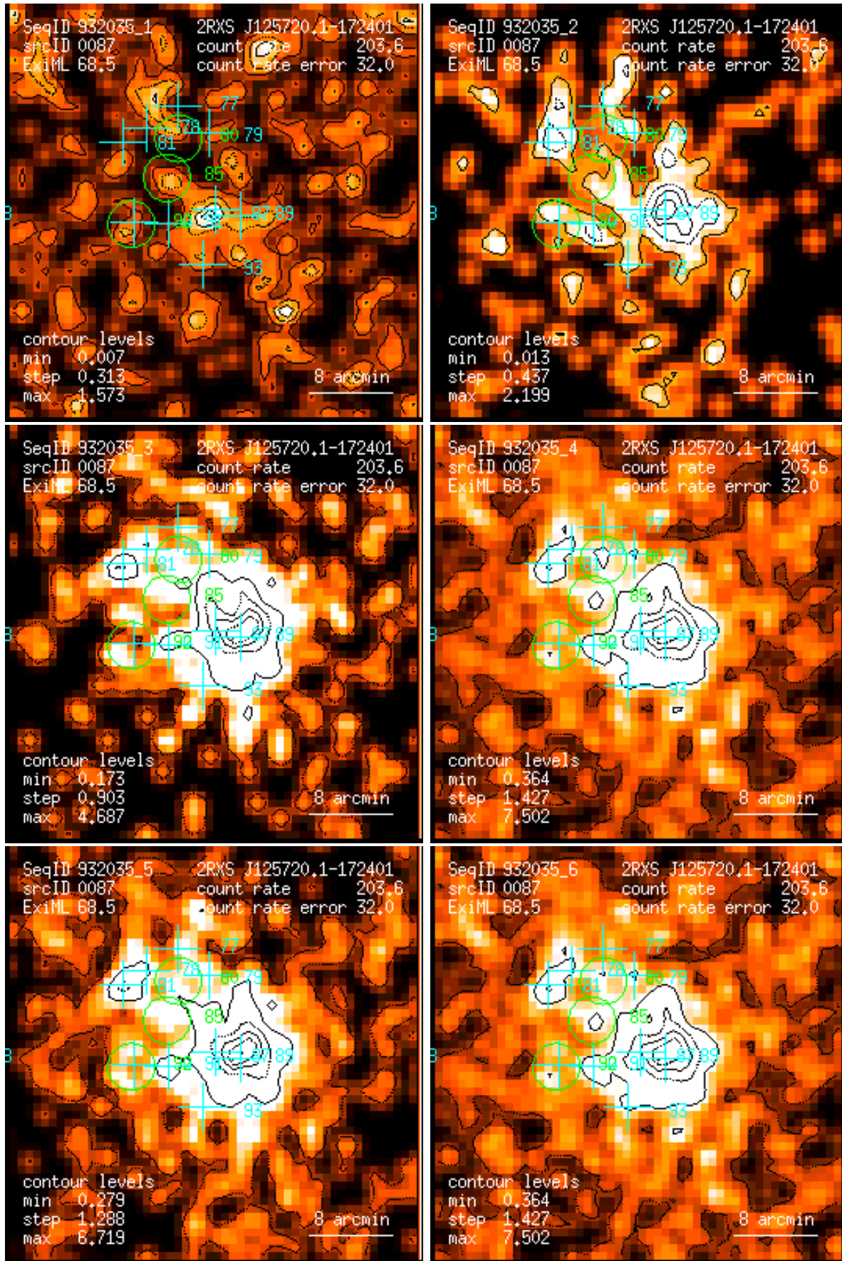
Figure 87: RASS 932035: detection 0087: band rate images, Gaussian filter: (1) PSPC channels 11 – 41, (2) 52 – 90, (3) 91 – 201, (4) 11 – 235, (5) 52 – 201, (6) 11 – 201. Broad band rates in counts/ks. Band rate contour levels in counts/ks/arcmin 2 .
