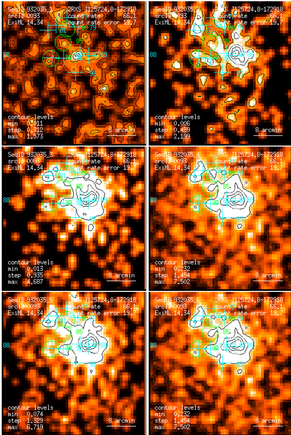
Figure 93: RASS 932035: detection 0093: band rate images, Gaussian filter: (1) PSPC channels 11 – 41, (2) 52 – 90, (3) 91 – 201, (4) 11 – 235, (5) 52 – 201, (6) 11 – 201. Broad band rates in counts/ks. Band rate contour levels in counts/ks/arcmin 2 .
