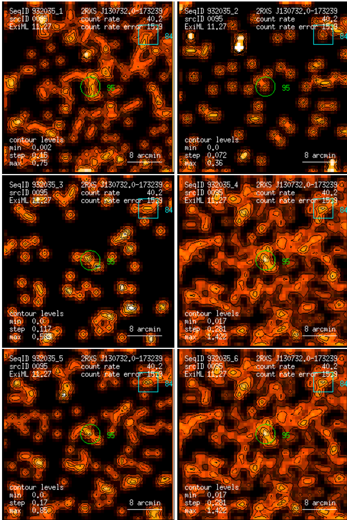
Figure 95: RASS 932035: detection 0095: band rate images, Gaussian filter: (1) PSPC channels 11 – 41, (2) 52 – 90, (3) 91 – 201, (4) 11 – 235, (5) 52 – 201, (6) 11 – 201. Broad band rates in counts/ks. Band rate contour levels in counts/ks/arcmin 2 .
