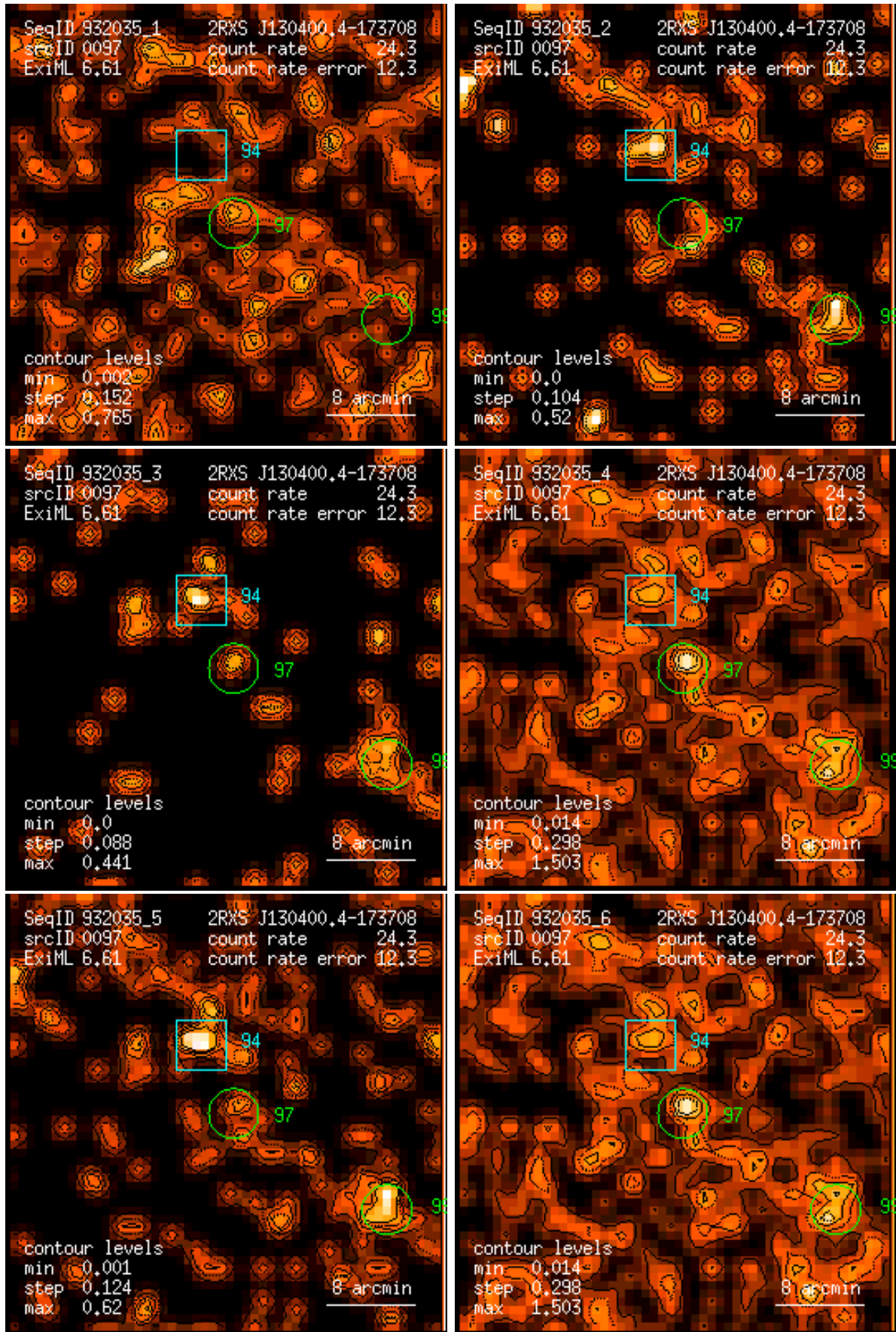
Figure 97: RASS 932035: detection 0097: band rate images, Gaussian filter: (1) PSPC channels 11 – 41, (2) 52 – 90, (3) 91 – 201, (4) 11 – 235, (5) 52 – 201, (6) 11 – 201. Broad band rates in counts/ks. Band rate contour levels in counts/ks/arcmin 2 .
