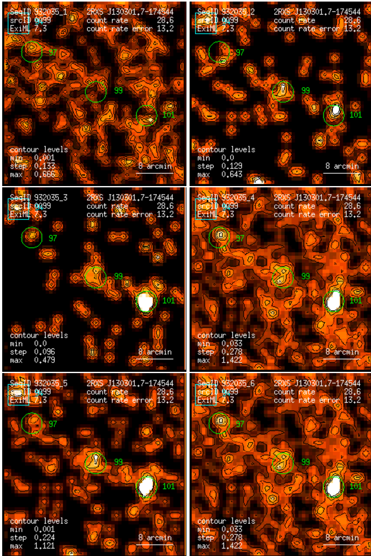
Figure 99: RASS 932035: detection 0099: band rate images, Gaussian filter: (1) PSPC channels 11 – 41, (2) 52 – 90, (3) 91 – 201, (4) 11 – 235, (5) 52 – 201, (6) 11 – 201. Broad band rates in counts/ks. Band rate contour levels in counts/ks/arcmin 2 .
