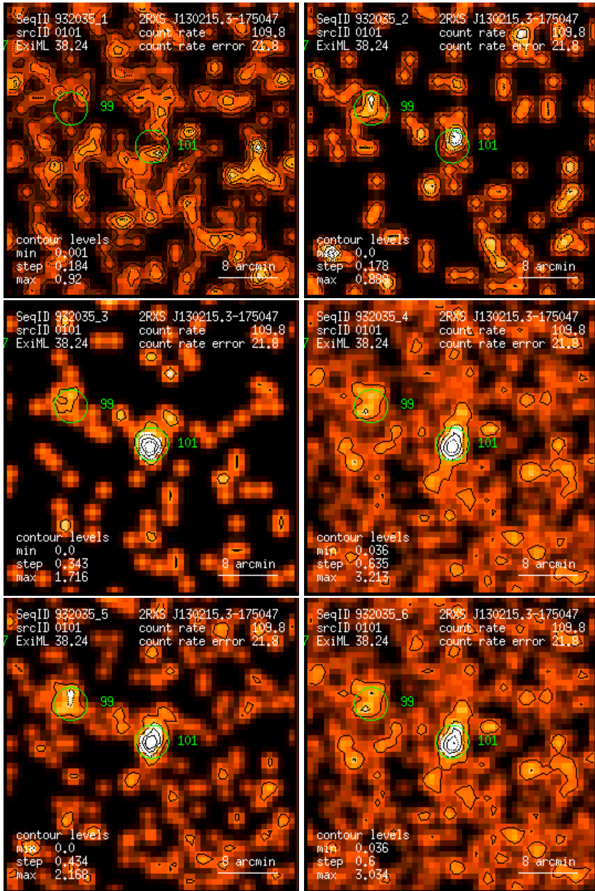
Figure 101: RASS 932035: detection 0101: band rate images, Gaussian filter: (1) PSPC channels 11 – 41, (2) 52 – 90, (3) 91 – 201, (4) 11 – 235, (5) 52 – 201, (6) 11 – 201. Broad band rates in counts/ks. Band rate contour levels in counts/ks/arcmin 2 .
