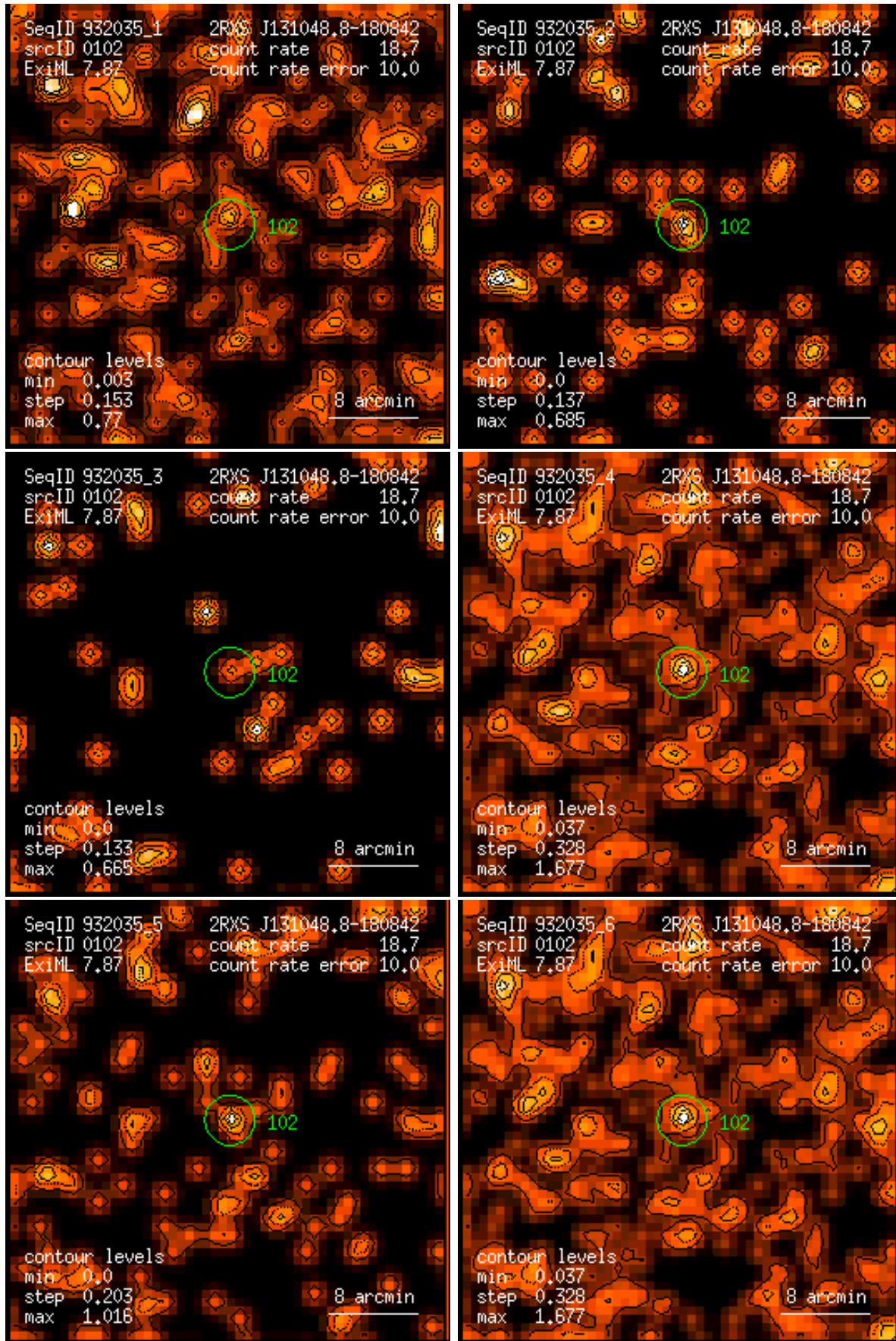
Figure 102: RASS 932035: detection 0102: band rate images, Gaussian filter: (1) PSPC channels 11 – 41, (2) 52 – 90, (3) 91 – 201, (4) 11 – 235, (5) 52 – 201, (6) 11 – 201. Broad band rates in counts/ks. Band rate contour levels in counts/ks/arcmin 2 .
