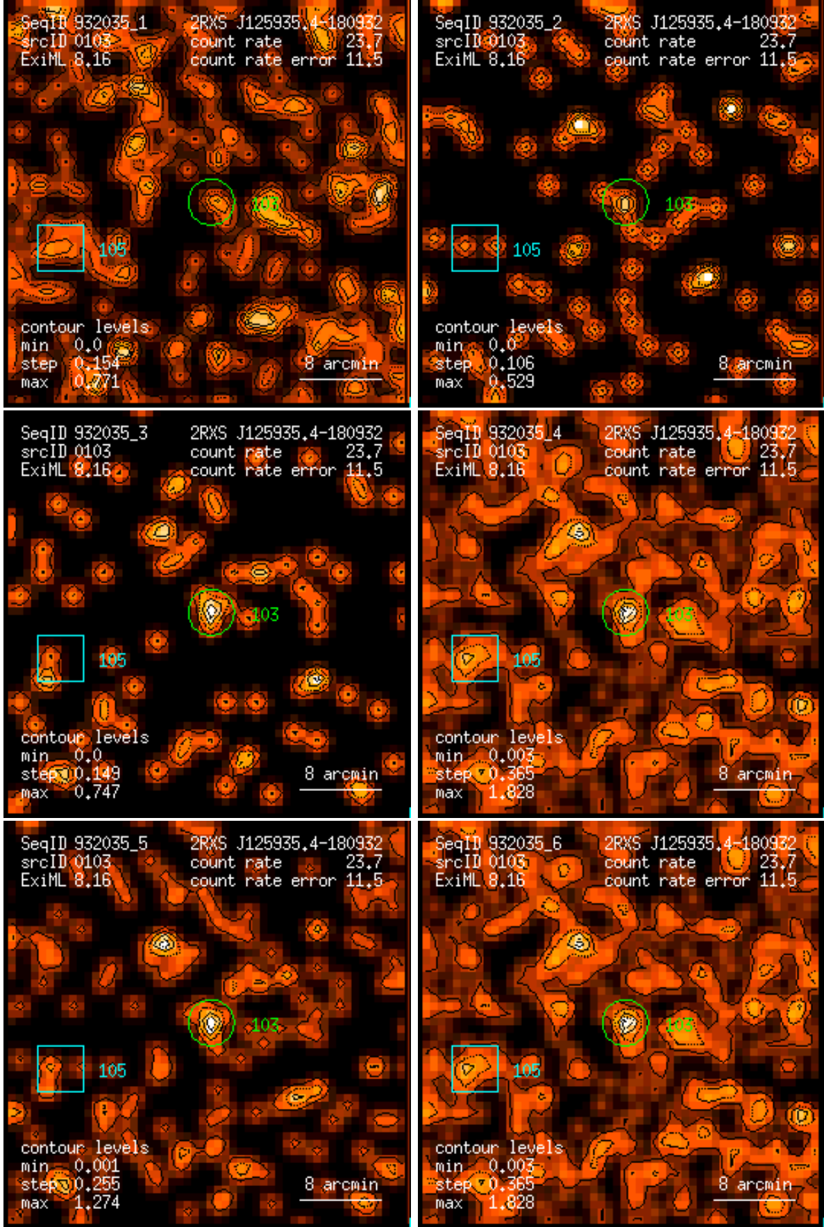
Figure 103: RASS 932035: detection 0103: band rate images, Gaussian filter: (1) PSPC channels 11 – 41, (2) 52 – 90, (3) 91 – 201, (4) 11 – 235, (5) 52 – 201, (6) 11 – 201. Broad band rates in counts/ks. Band rate contour levels in counts/ks/arcmin 2 .
