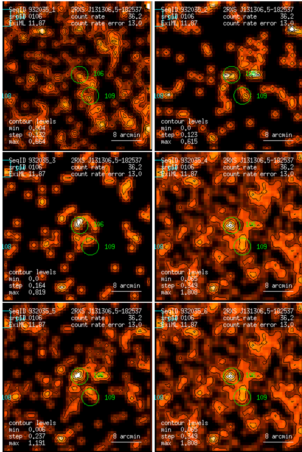
Figure 106: RASS 932035: detection 0106: band rate images, Gaussian filter: (1) PSPC channels 11 – 41, (2) 52 – 90, (3) 91 – 201, (4) 11 – 235, (5) 52 – 201, (6) 11 – 201. Broad band rates in counts/ks. Band rate contour levels in counts/ks/arcmin 2 .
