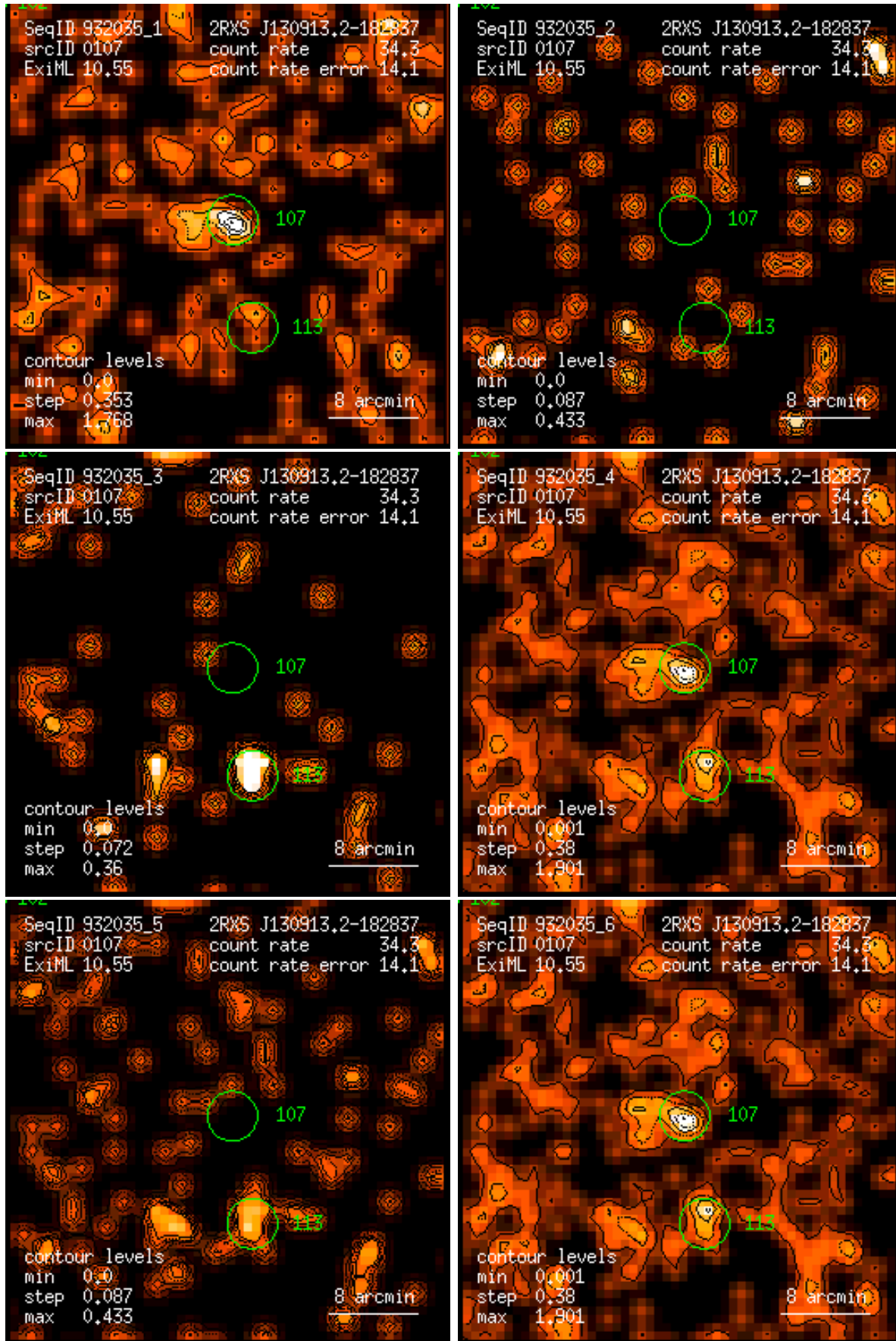
Figure 107: RASS 932035: detection 0107: band rate images, Gaussian filter: (1) PSPC channels 11 – 41, (2) 52 – 90, (3) 91 – 201, (4) 11 – 235, (5) 52 – 201, (6) 11 – 201. Broad band rates in counts/ks. Band rate contour levels in counts/ks/arcmin 2 .
