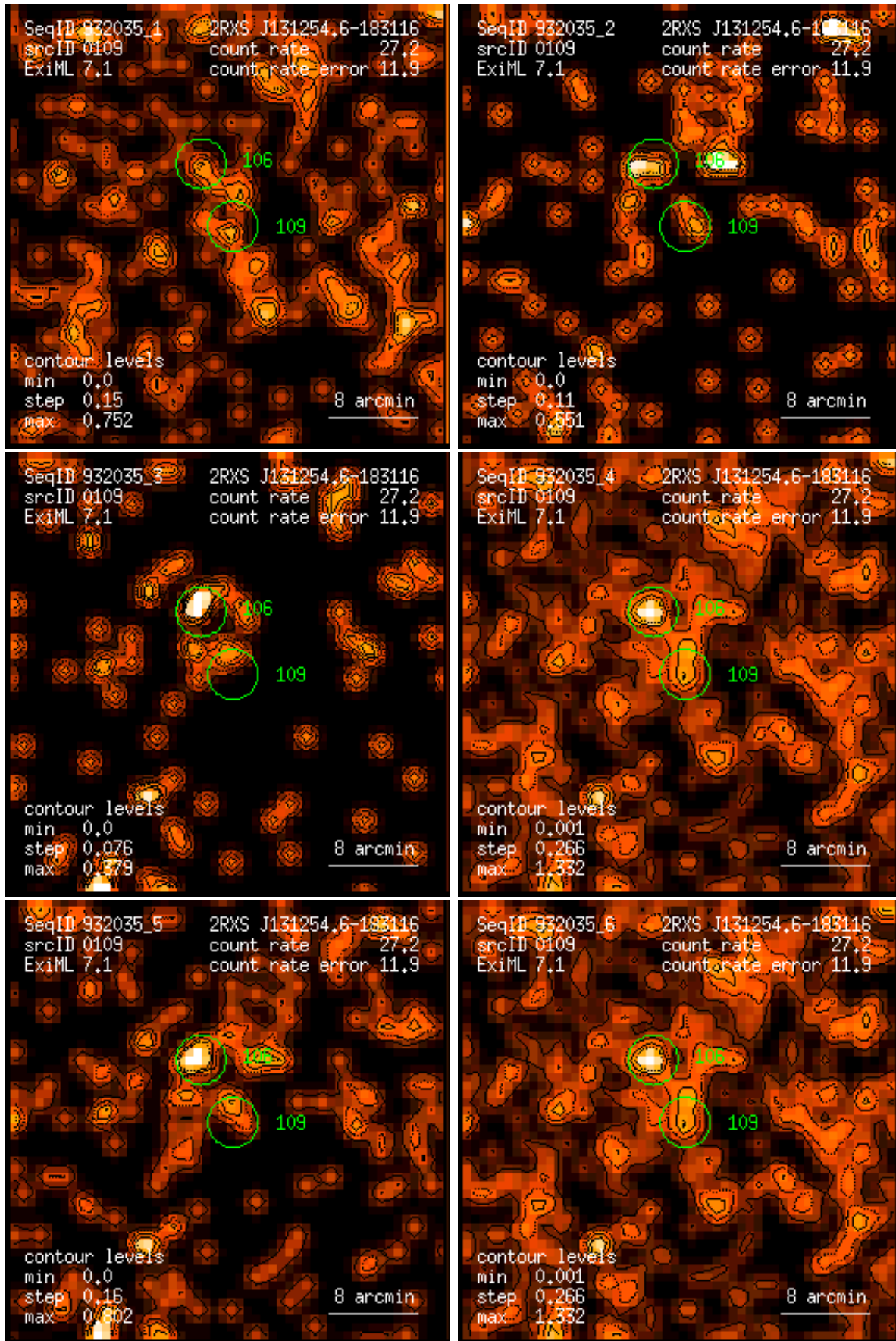
Figure 109: RASS 932035: detection 0109: band rate images, Gaussian filter: (1) PSPC channels 11 – 41, (2) 52 – 90, (3) 91 – 201, (4) 11 – 235, (5) 52 – 201, (6) 11 – 201. Broad band rates in counts/ks. Band rate contour levels in counts/ks/arcmin 2 .
