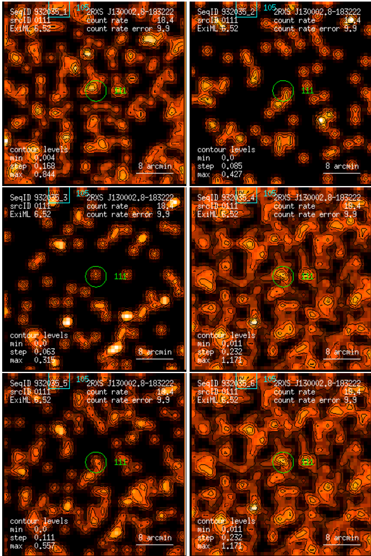
Figure 111: RASS 932035: detection 0111: band rate images, Gaussian filter: (1) PSPC channels 11 – 41, (2) 52 – 90, (3) 91 – 201, (4) 11 – 235, (5) 52 – 201, (6) 11 – 201. Broad band rates in counts/ks. Band rate contour levels in counts/ks/arcmin 2 .
