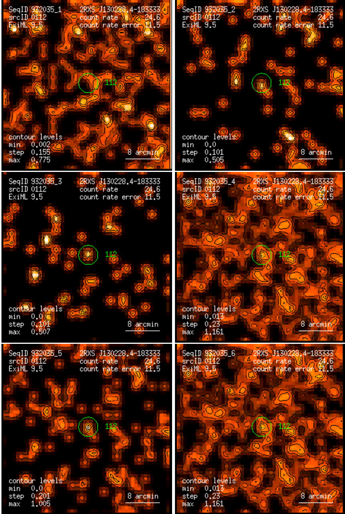
Figure 112: RASS 932035: detection 0112: band rate images, Gaussian filter: (1) PSPC channels 11 – 41, (2) 52 – 90, (3) 91 – 201, (4) 11 – 235, (5) 52 – 201, (6) 11 – 201. Broad band rates in counts/ks. Band rate contour levels in counts/ks/arcmin 2 .
