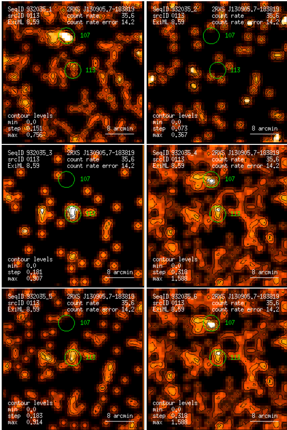
Figure 113: RASS 932035: detection 0113: band rate images, Gaussian filter: (1) PSPC channels 11 – 41, (2) 52 – 90, (3) 91 – 201, (4) 11 – 235, (5) 52 – 201, (6) 11 – 201. Broad band rates in counts/ks. Band rate contour levels in counts/ks/arcmin 2 .
