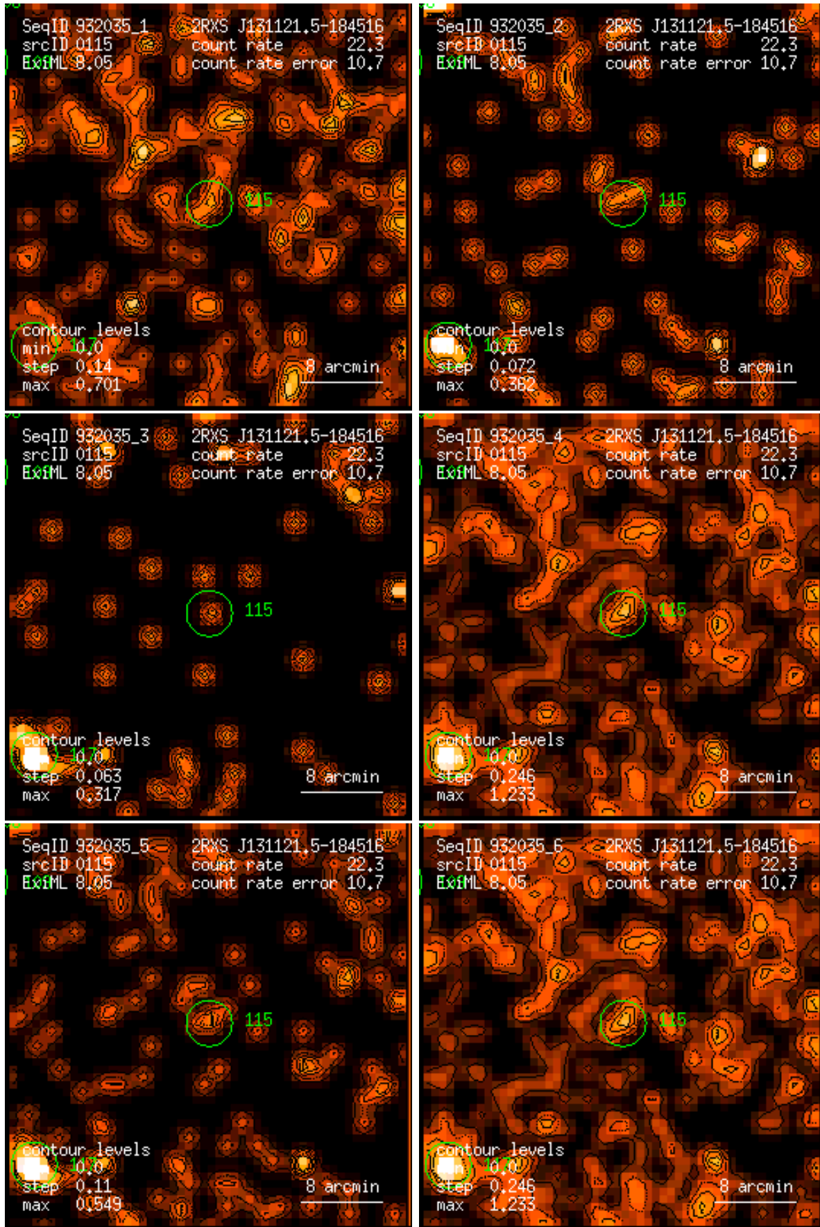
Figure 115: RASS 932035: detection 0115: band rate images, Gaussian filter: (1) PSPC channels 11 – 41, (2) 52 – 90, (3) 91 – 201, (4) 11 – 235, (5) 52 – 201, (6) 11 – 201. Broad band rates in counts/ks. Band rate contour levels in counts/ks/arcmin 2 .
