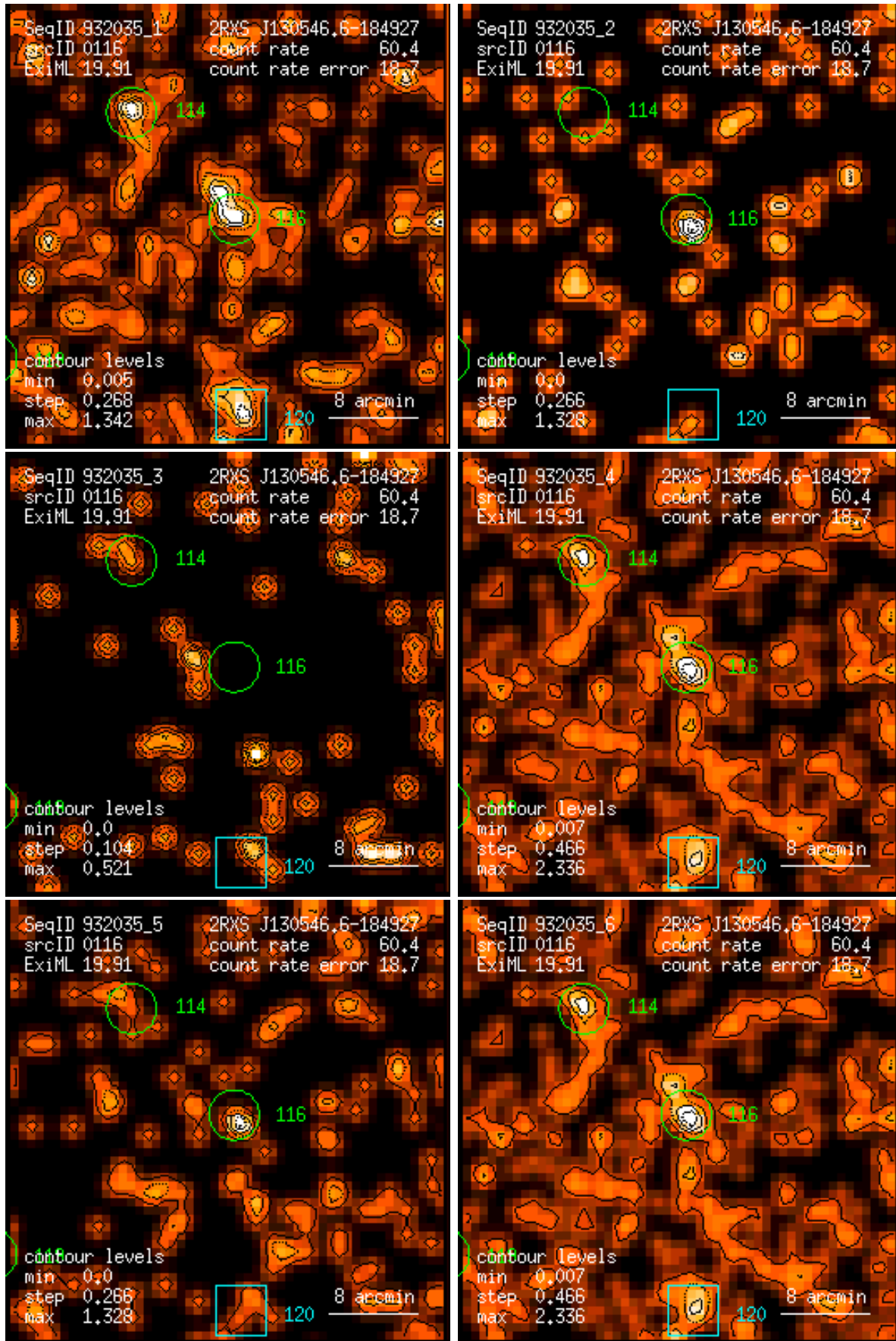
Figure 116: RASS 932035: detection 0116: band rate images, Gaussian filter: (1) PSPC channels 11 – 41, (2) 52 – 90, (3) 91 – 201, (4) 11 – 235, (5) 52 – 201, (6) 11 – 201. Broad band rates in counts/ks. Band rate contour levels in counts/ks/arcmin 2 .
