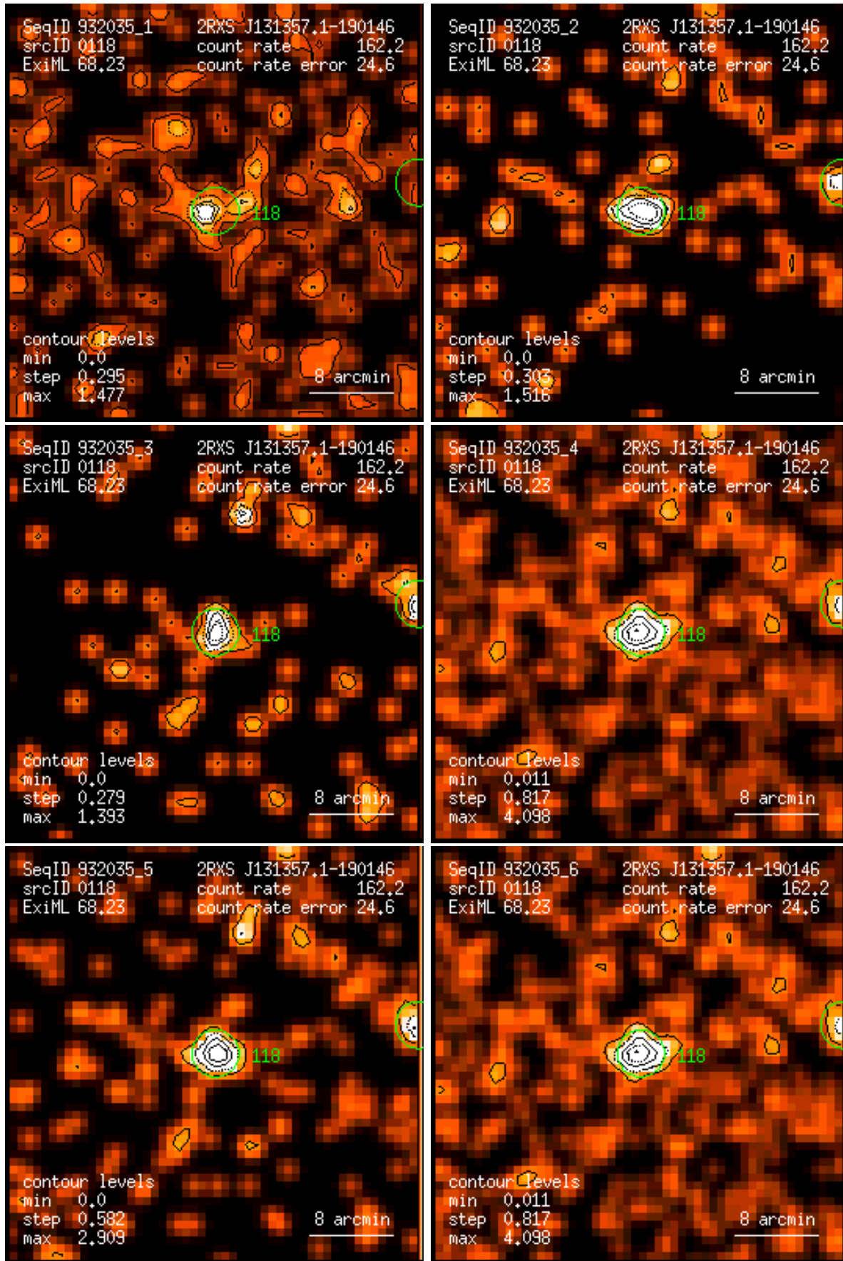
Figure 118: RASS 932035: detection 0118: band rate images, Gaussian filter: (1) PSPC channels 11 – 41, (2) 52 – 90, (3) 91 – 201, (4) 11 – 235, (5) 52 – 201, (6) 11 – 201. Broad band rates in counts/ks. Band rate contour levels in counts/ks/arcmin 2 .
